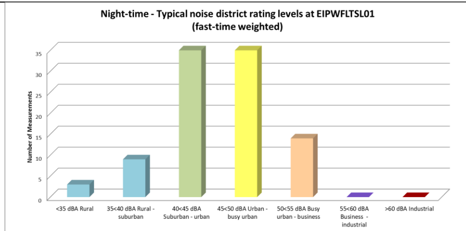
Figure 4-6: Classification of night-time measurements in typical noise districts at EIPWFLTSL01
