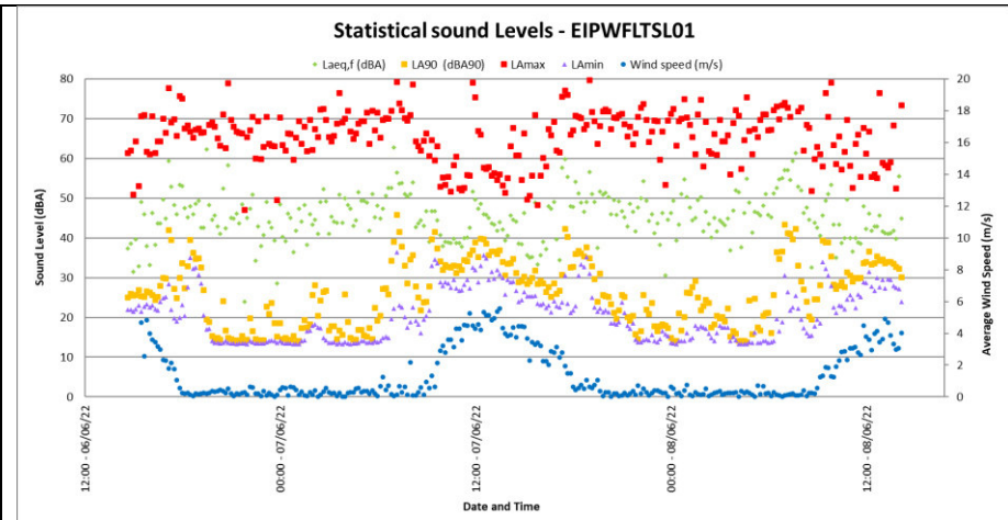
Figure 4-5: Maximum, minimum and Statistical sound levels at EIPWFLTSL01
