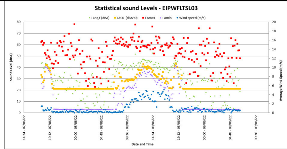
Figure 4-13: Maximum, minimum and Statistical sound levels at EIPWFLTSL03
