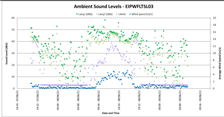
Figure 4-12: Ambient Sound Levels at EIPWFLTSL03
