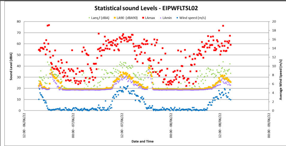
Figure 4-9: Maximum, minimum and statistical values at EIPWFLTSL02
