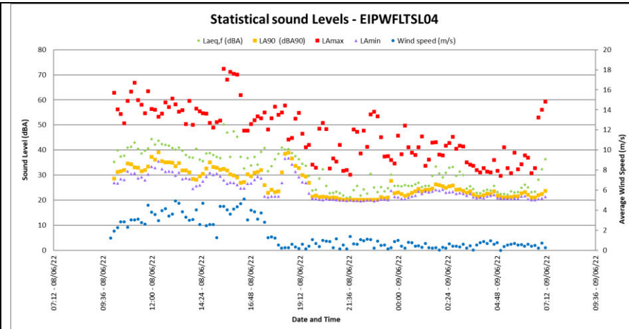
Figure 4-17: Maximum, minimum and Statistical sound levels at EIPWFLTSL04
