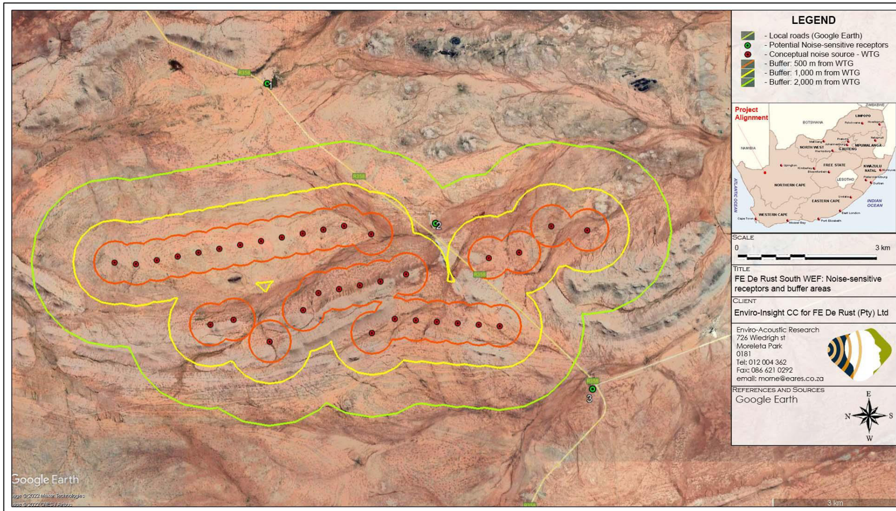
Figure 2-2: Study area and potential noise-sensitive receptors close to FE De Rust South WEF
