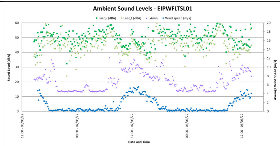
Figure 4-4: Ambient Sound Levels at EIPWFLTSL01
