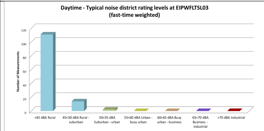
Figure 4-15: Classification of daytime measurements in typical noise districts at EIPWFLTSL03
