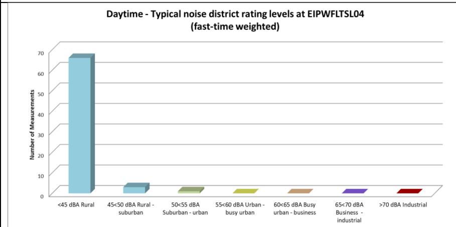
Figure 4-19: Classification of daytime measurements in typical noise districts at EIPWFLTSL04
