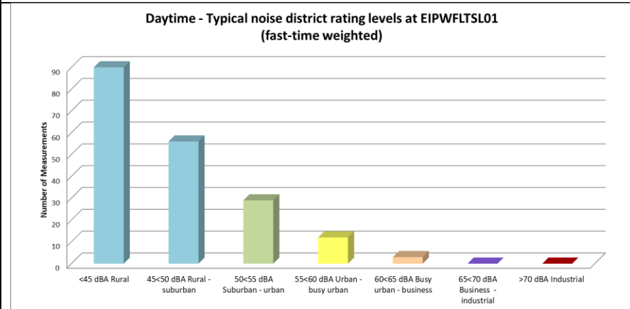
Figure 4-7: Classification of daytime measurements in typical noise districts at EIPWFLTSL01
