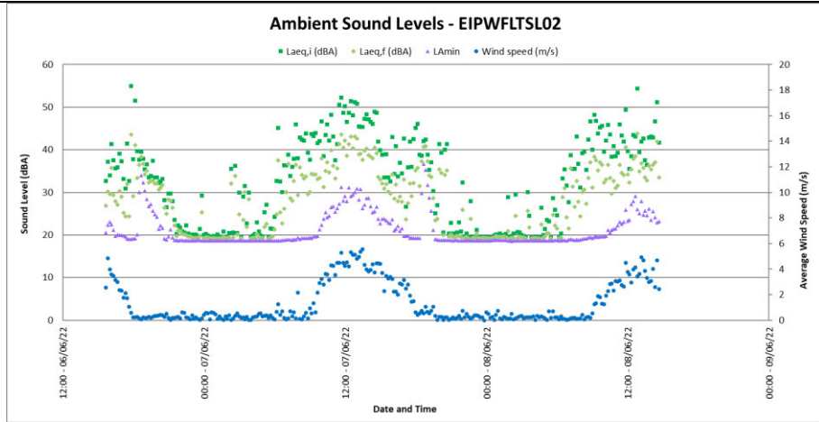
Figure 4-8: Ambient sound levels at EIPWFLTSL02
