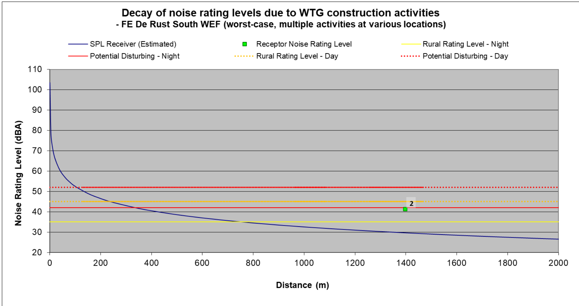
Figure 9-3: Projected conceptual construction noise levels – FE De Rust South WEF
