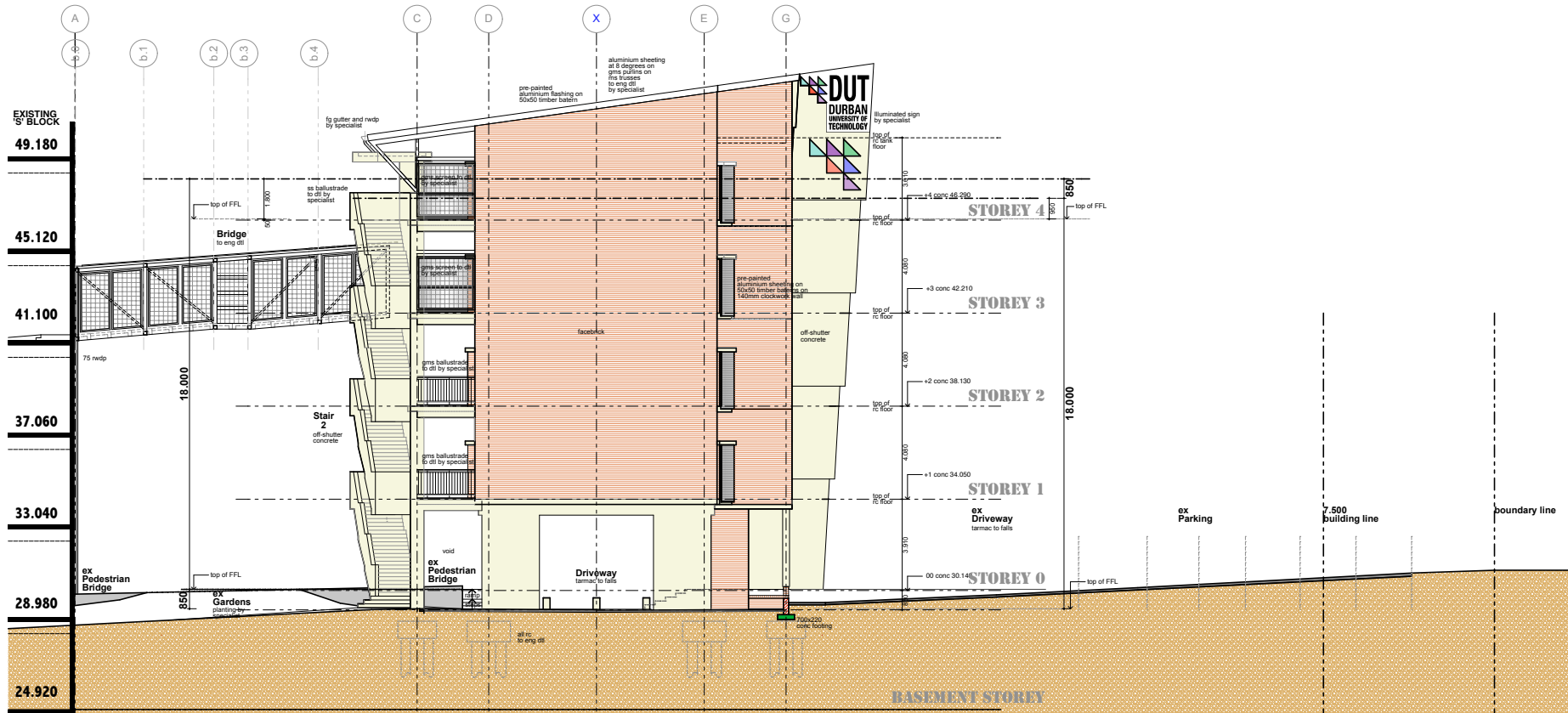
North Elevation
