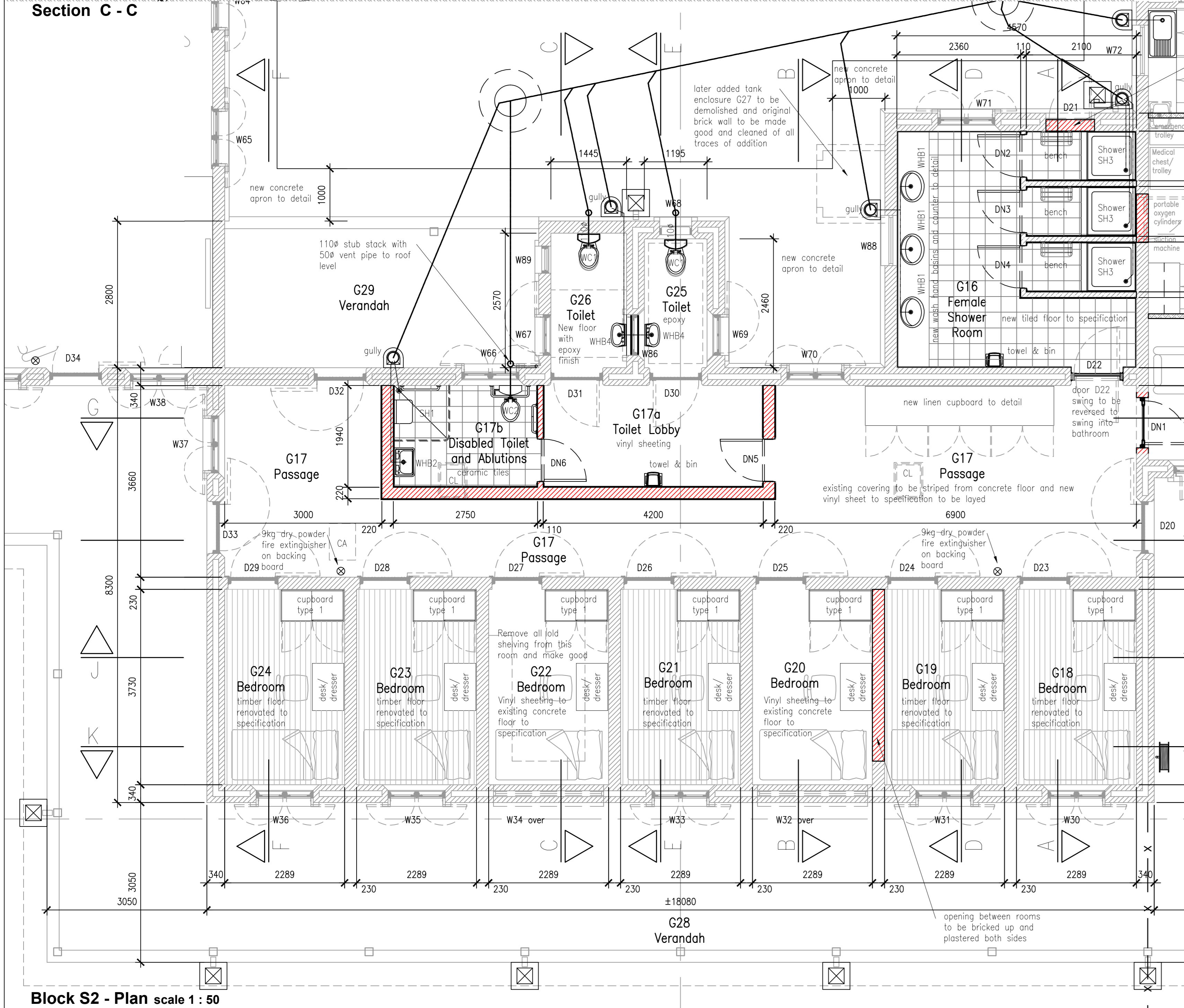
Block S2 - Plan scale 1:50
