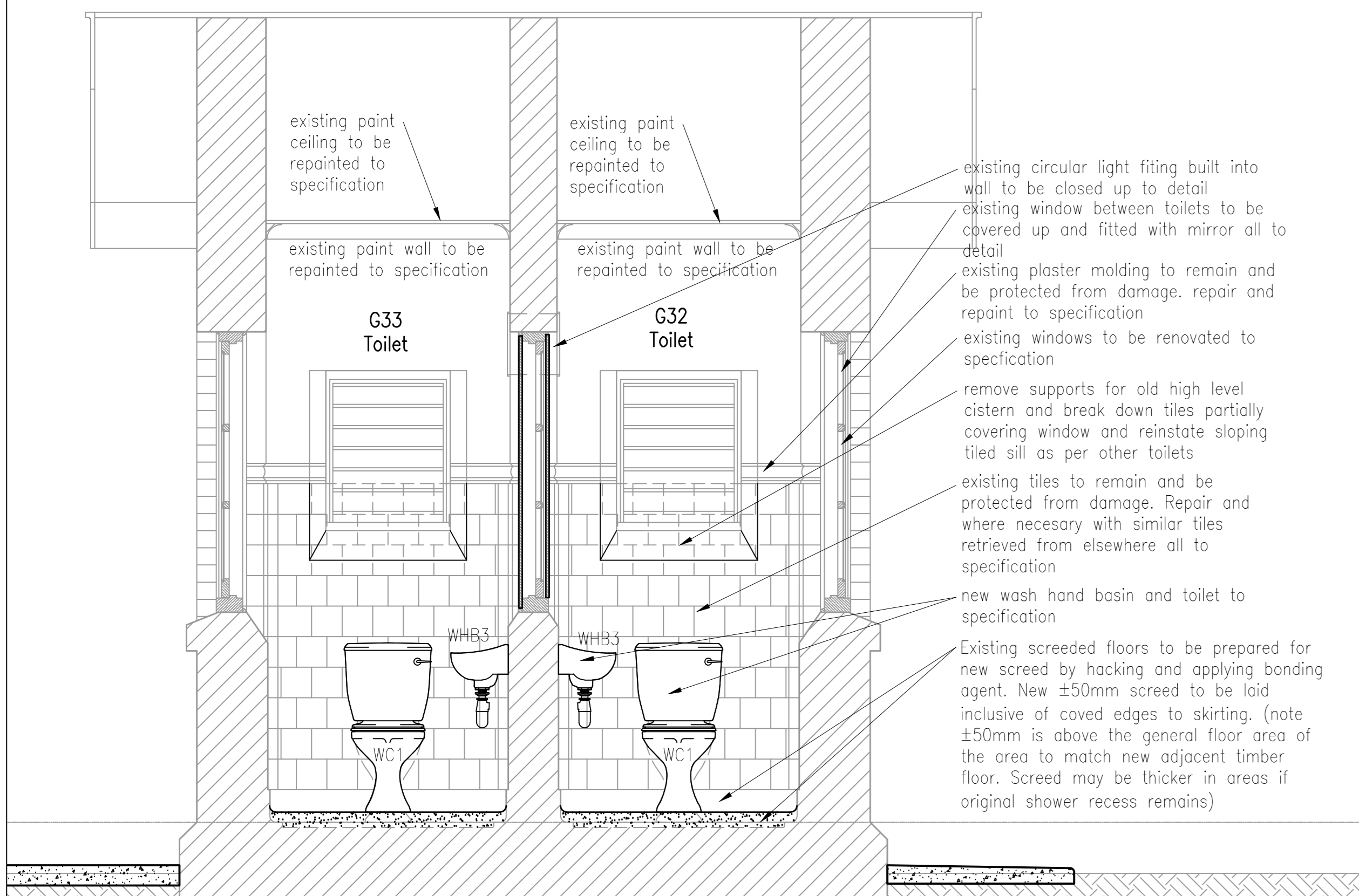
View 3 scale 1 : 20
