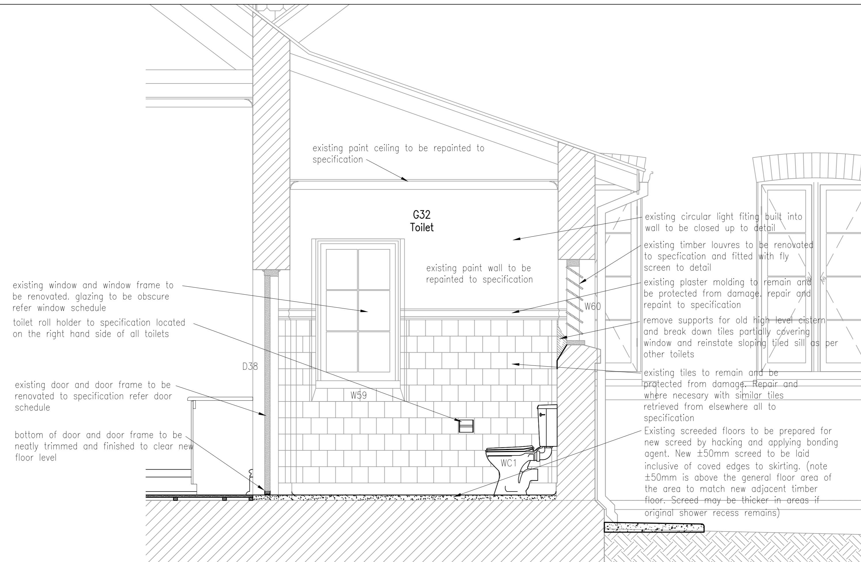
View 2 Toilet G32 scale 1 : 20 view 4 toilet G33 mirror image
