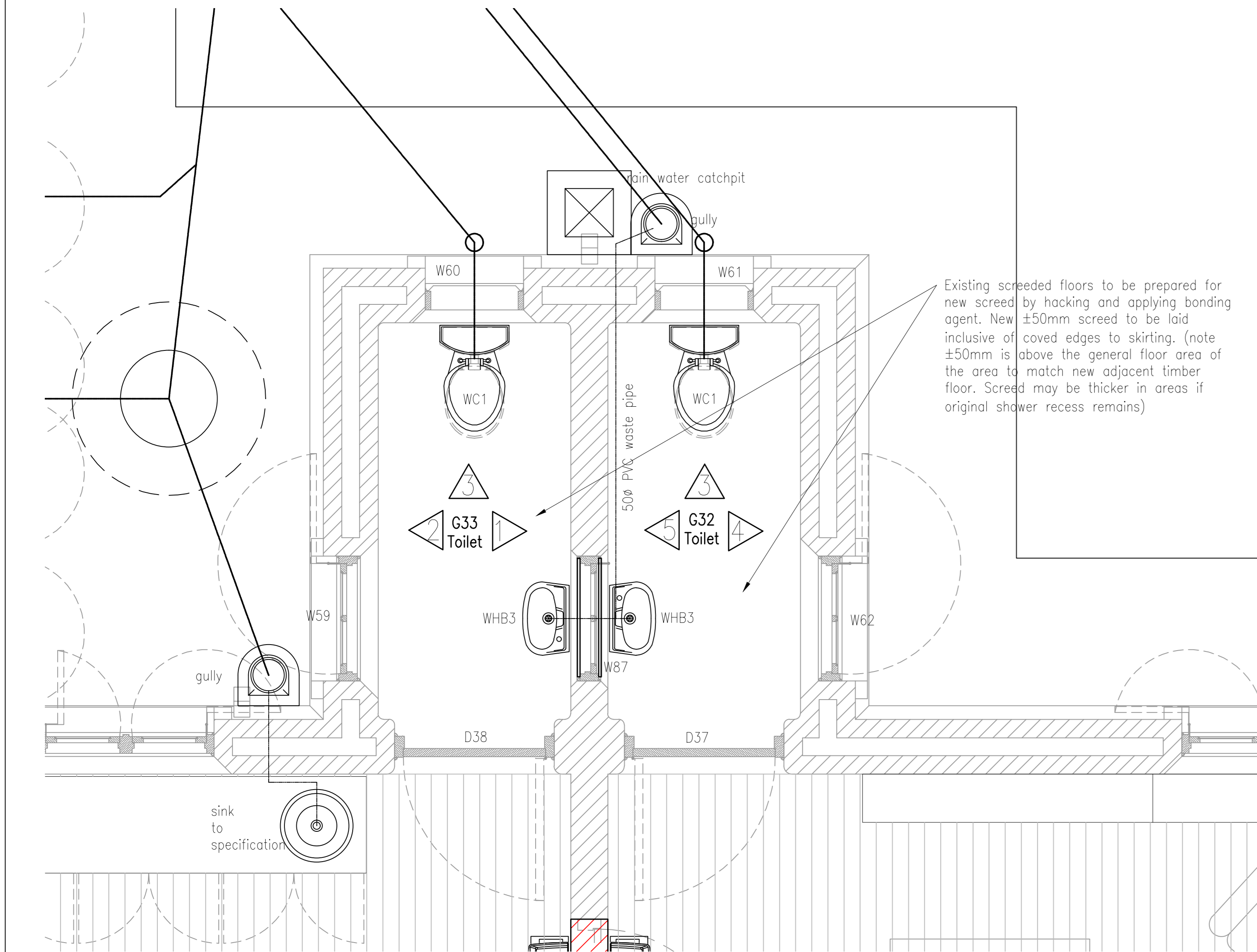
Plan Toilets G32 and G33 Block S3 scale 1 : 20
