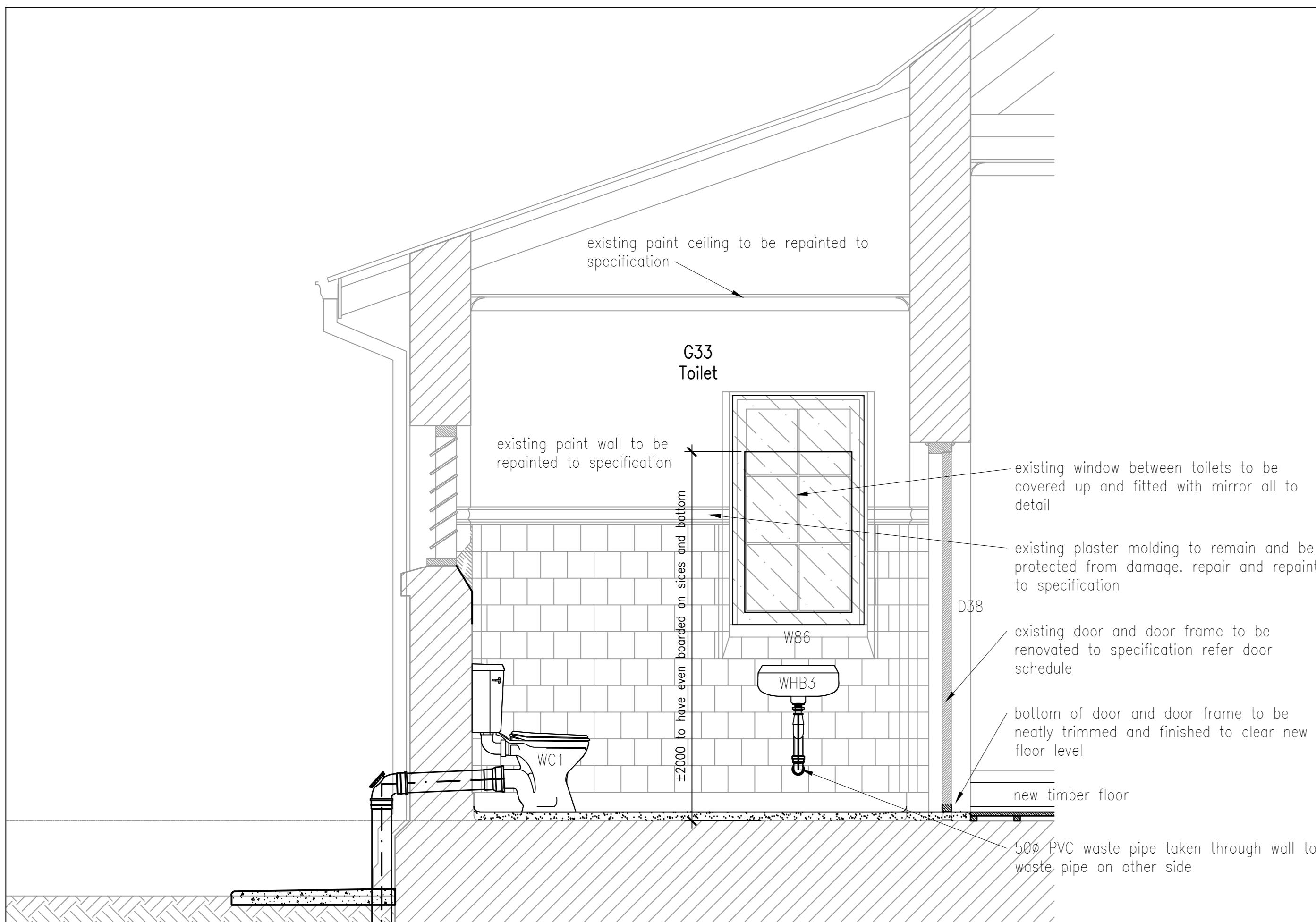
View 1 Toilet G33 scale 1 : 20
