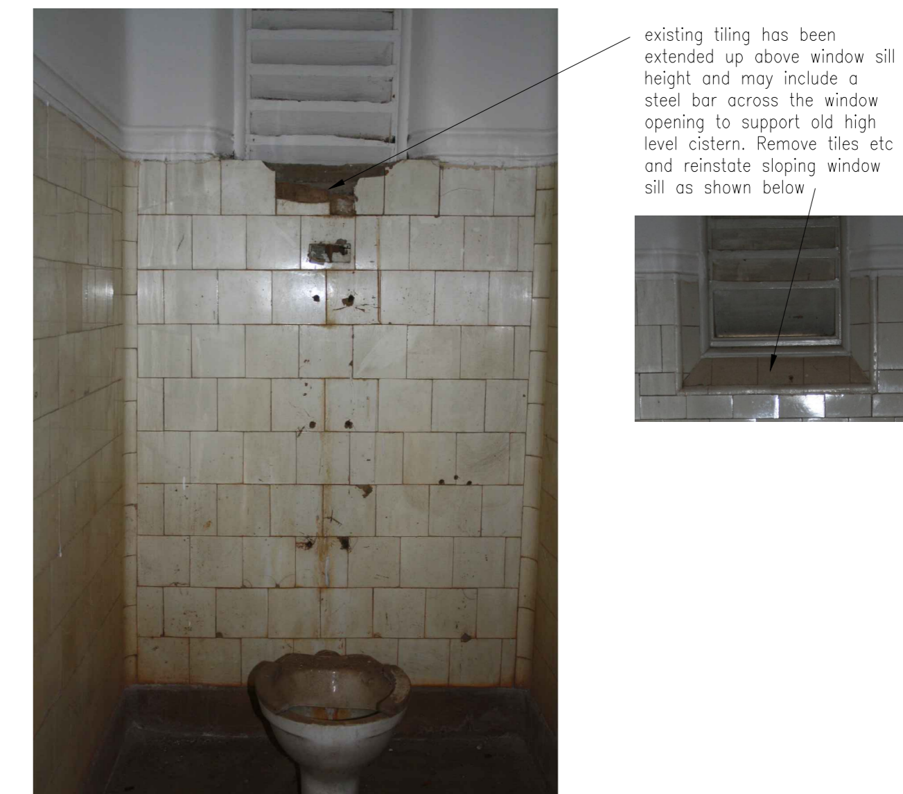
View Toilet G32 showing window sill problem
