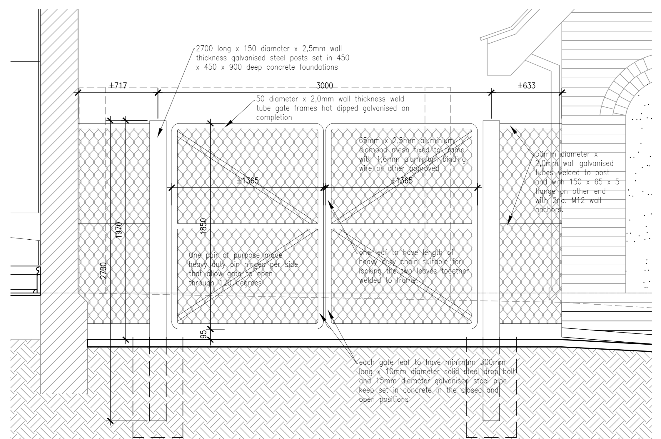
Detailed Elevation Gate scale 1 : 20
