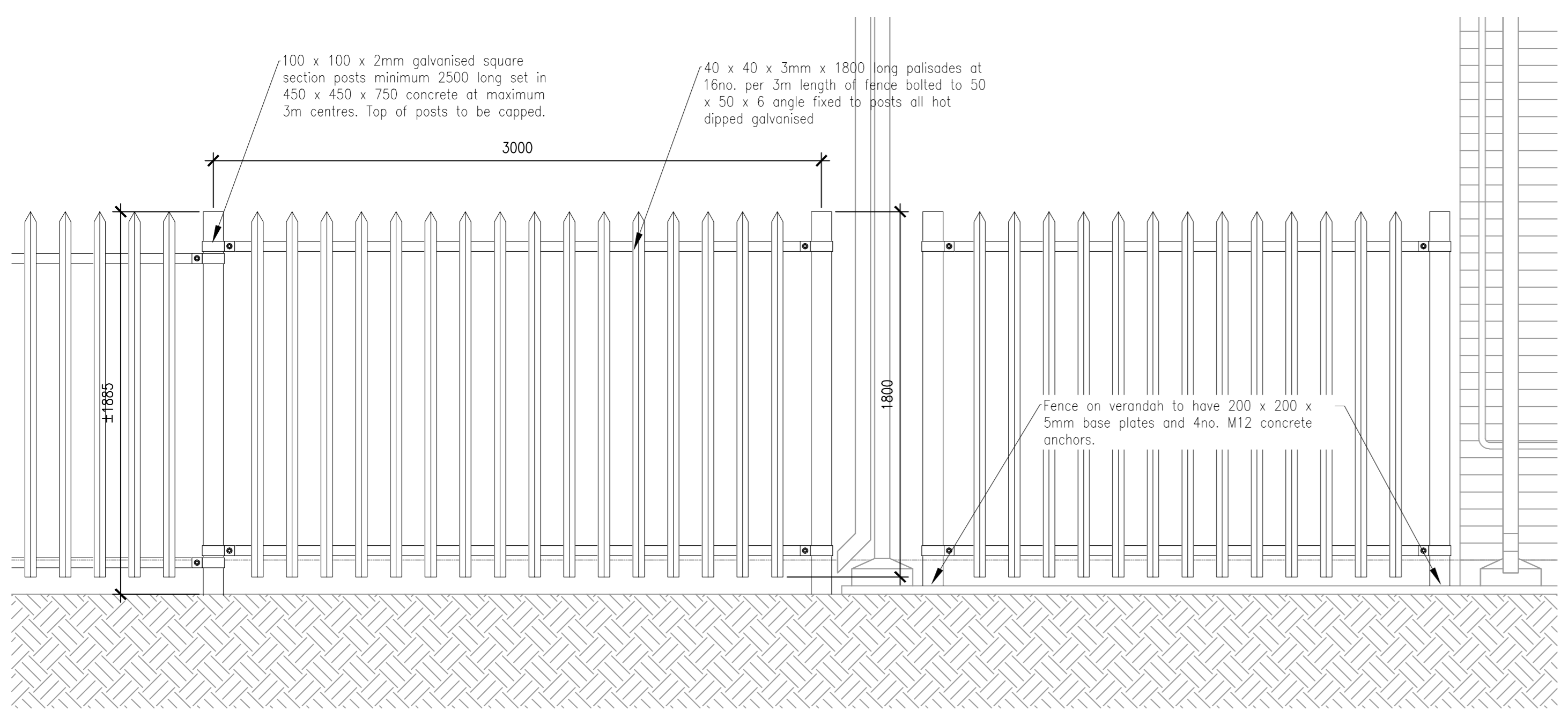
Typical Fence Elevation and Detail scale 1 : 20
