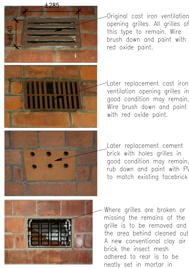
External Air Grilles / Blocks scale 1 : 10
