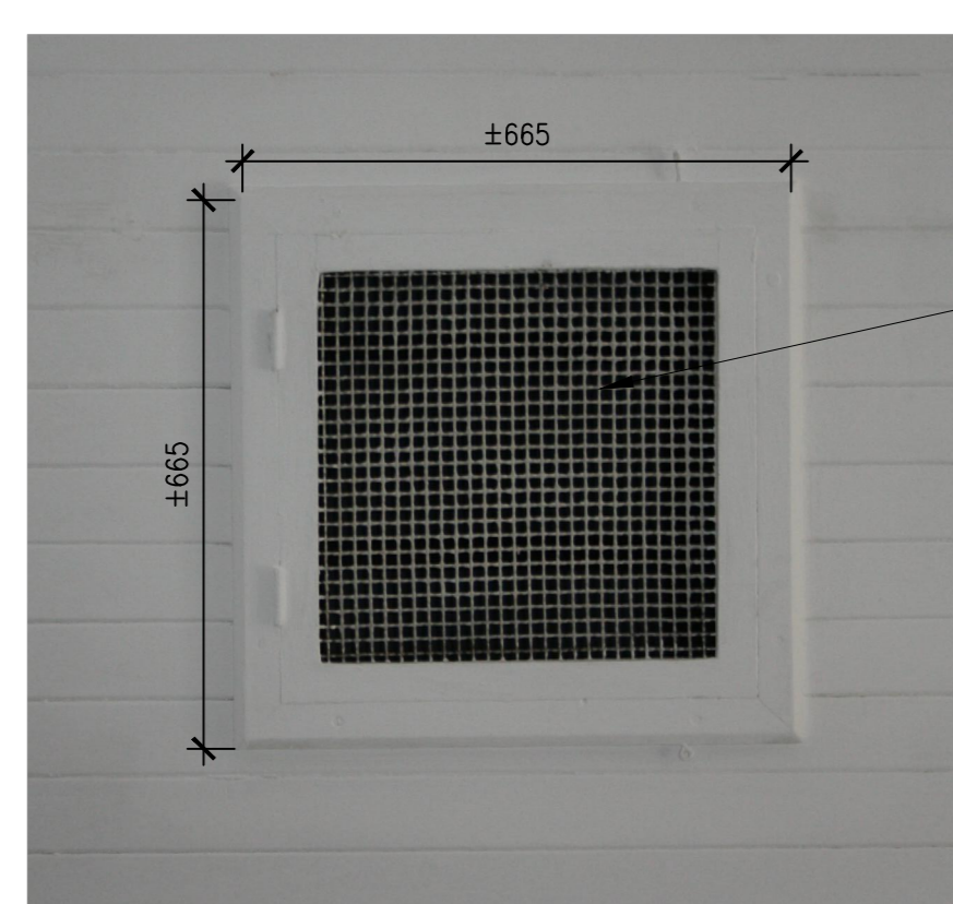
Internal Wall and Ceiling Air grilles and Original light fittings scale 1 : 10
