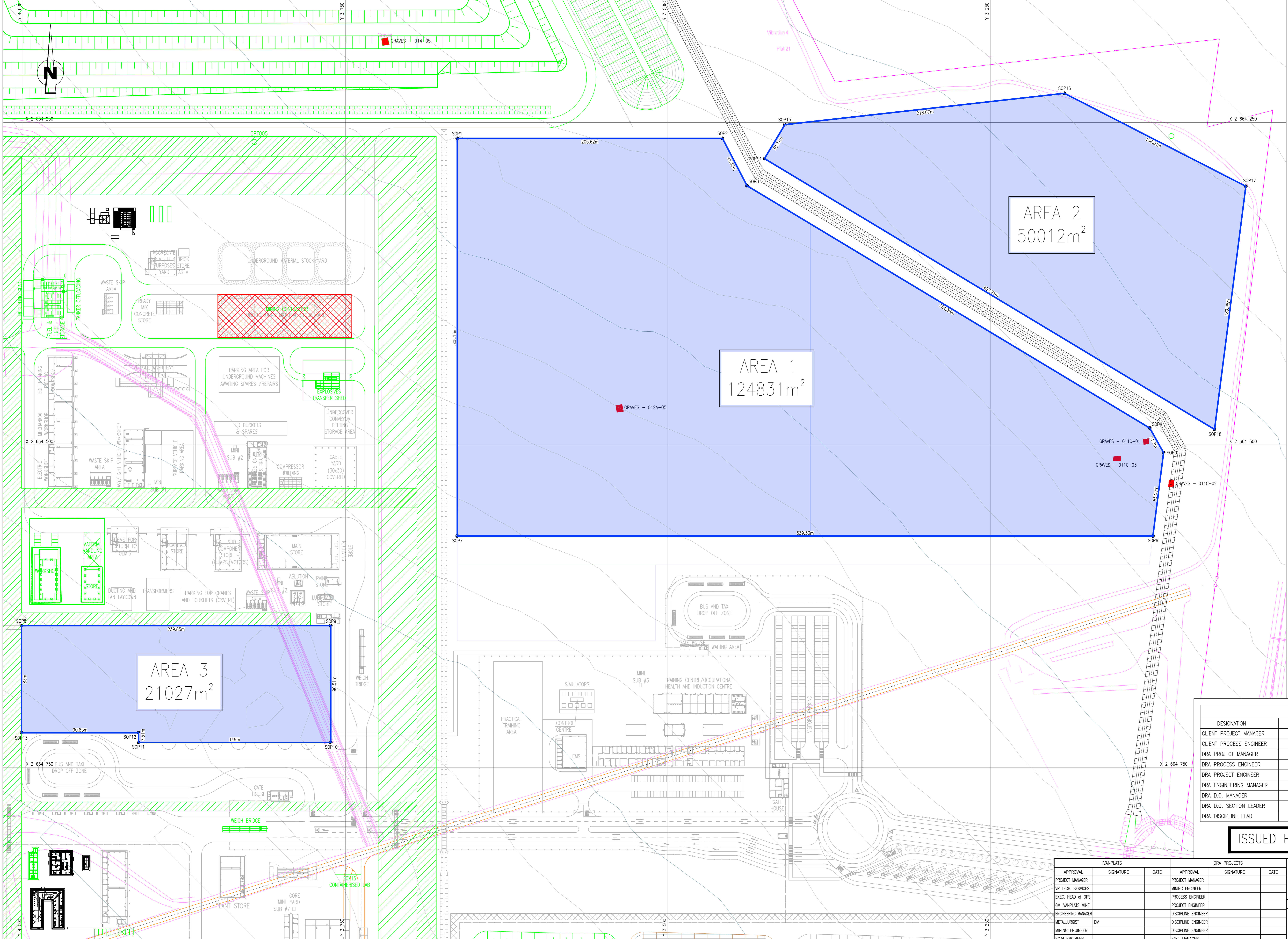
MAIN SOLAR PLANT LAYOUT SCALE 1:1000
