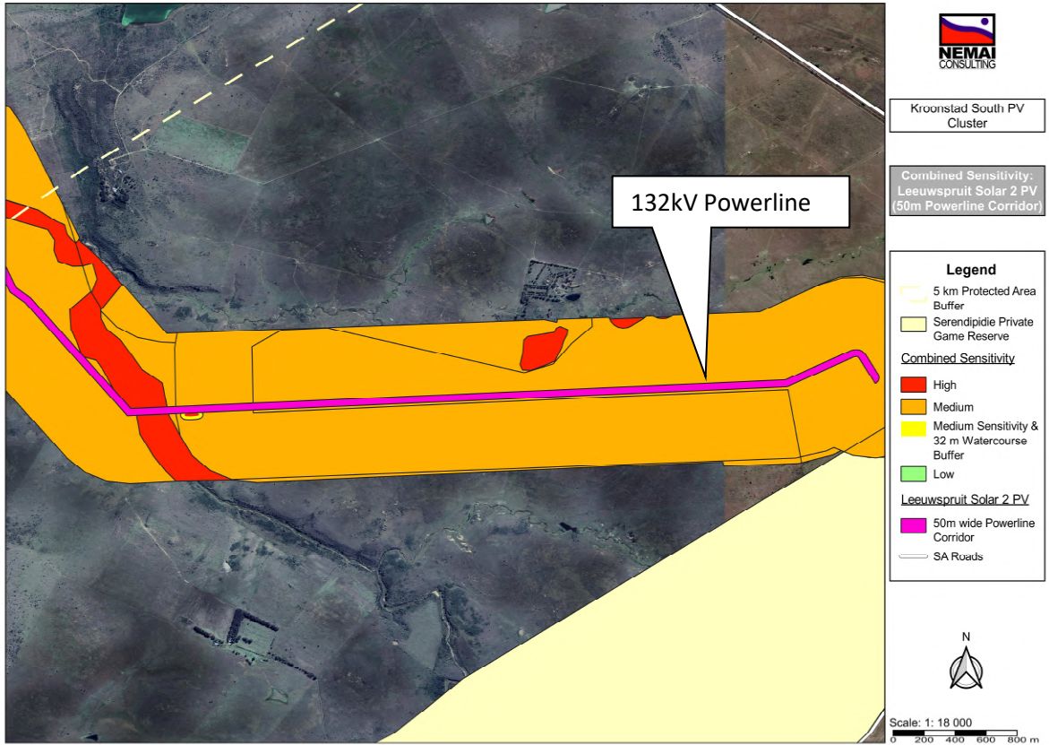
Figure 5: Sensitivity map based on Specialist Studies for Layout Alternative 2 eastern section of powerline (preferred alternative)
