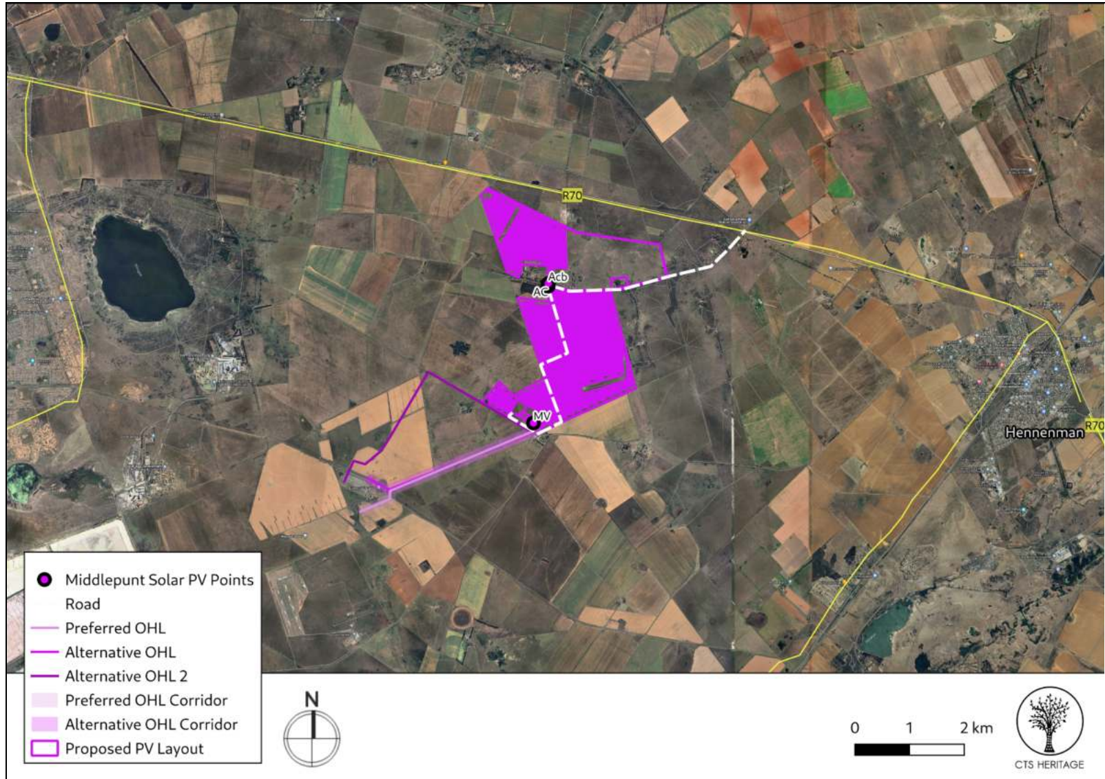
Figure 1.1: The proposed development layout of the Middlepunt SPP assessed in this report
