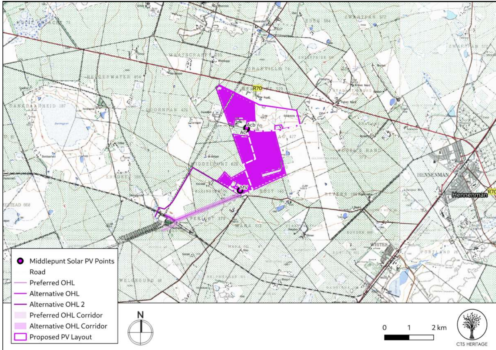
Figure 1.5: The proposed development layout on an extract of the 1:50 000 Topo Map of the Middlepunt SPP
