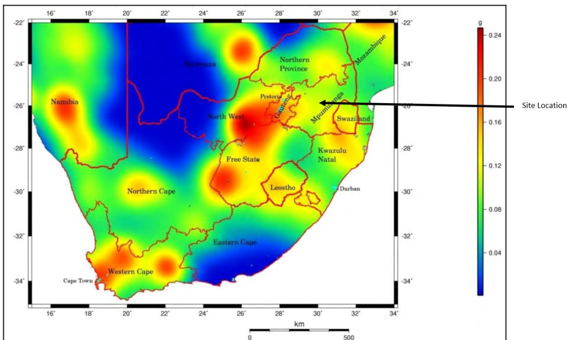
Figure 6: Seismic Hazard Map of South Africa
