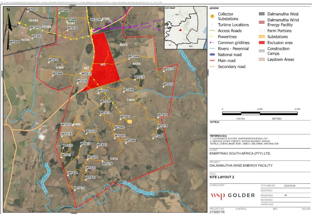
Figure 8: Position of turbines in the Southern Portion of the Site Plan
