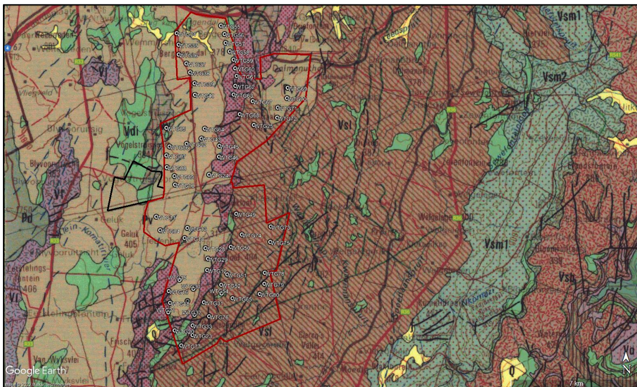
Figure 5: Geology Map of the Project Site
