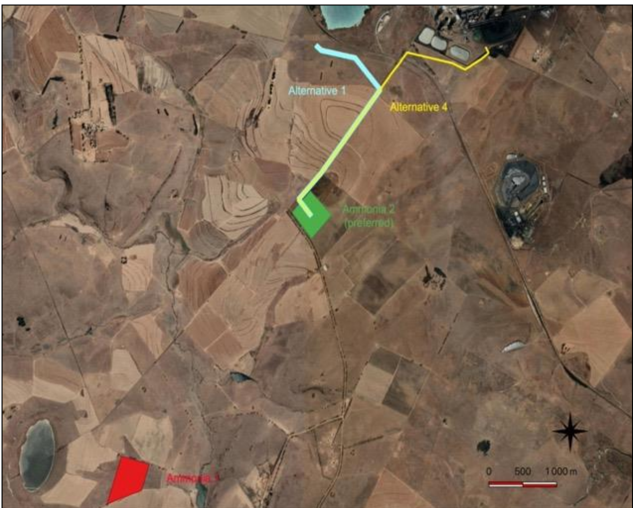
Figure 10: Pipeline alternatives for Ammonia 2.
