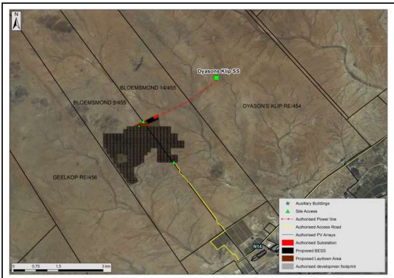
Figure 1. Revised lay out indicating the proposed BESS (Cape EA Prac) .
