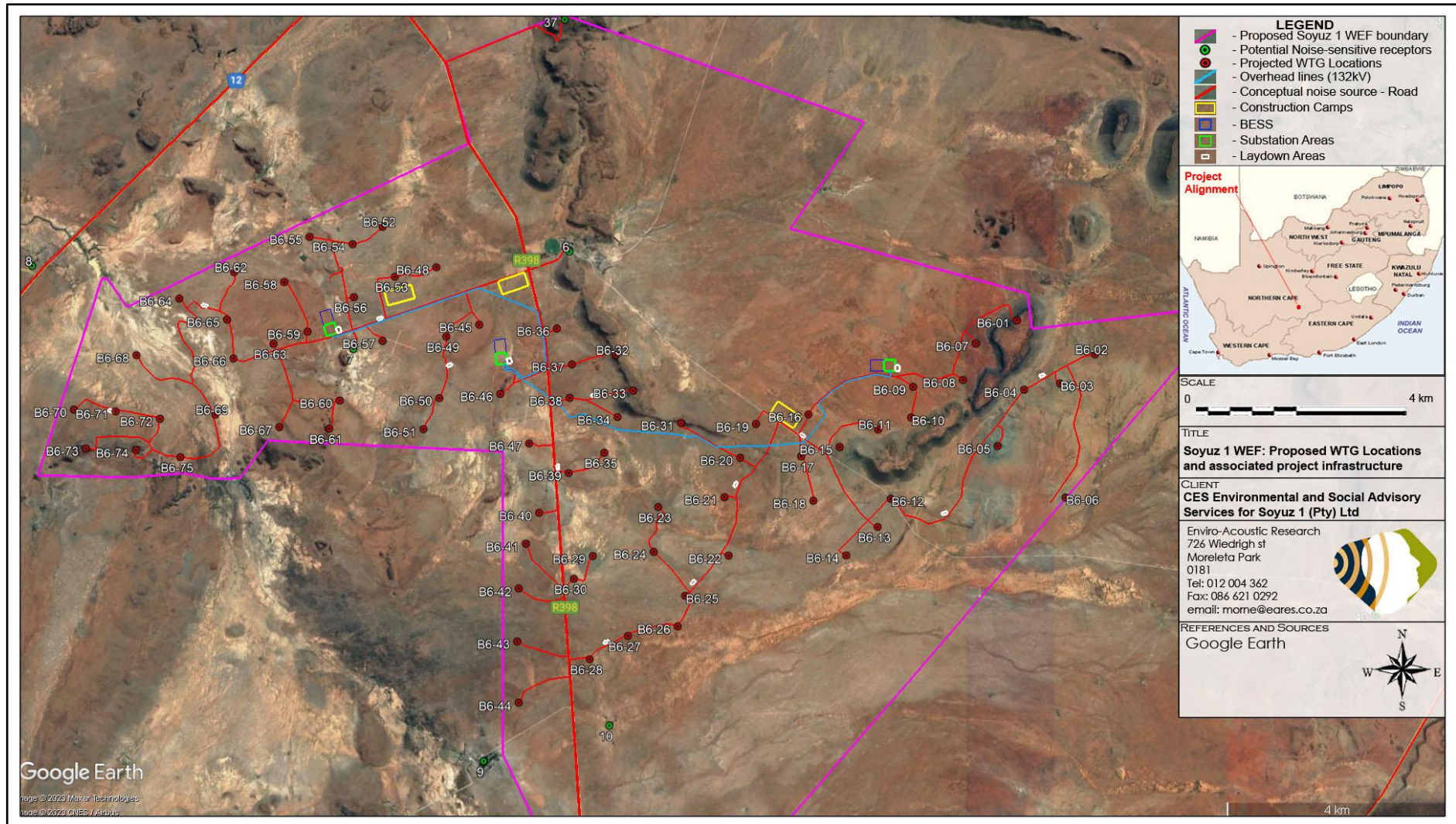
Figure 9-1: WTG locations and associated infrastructure for the proposed Soyuz 1 WEF
