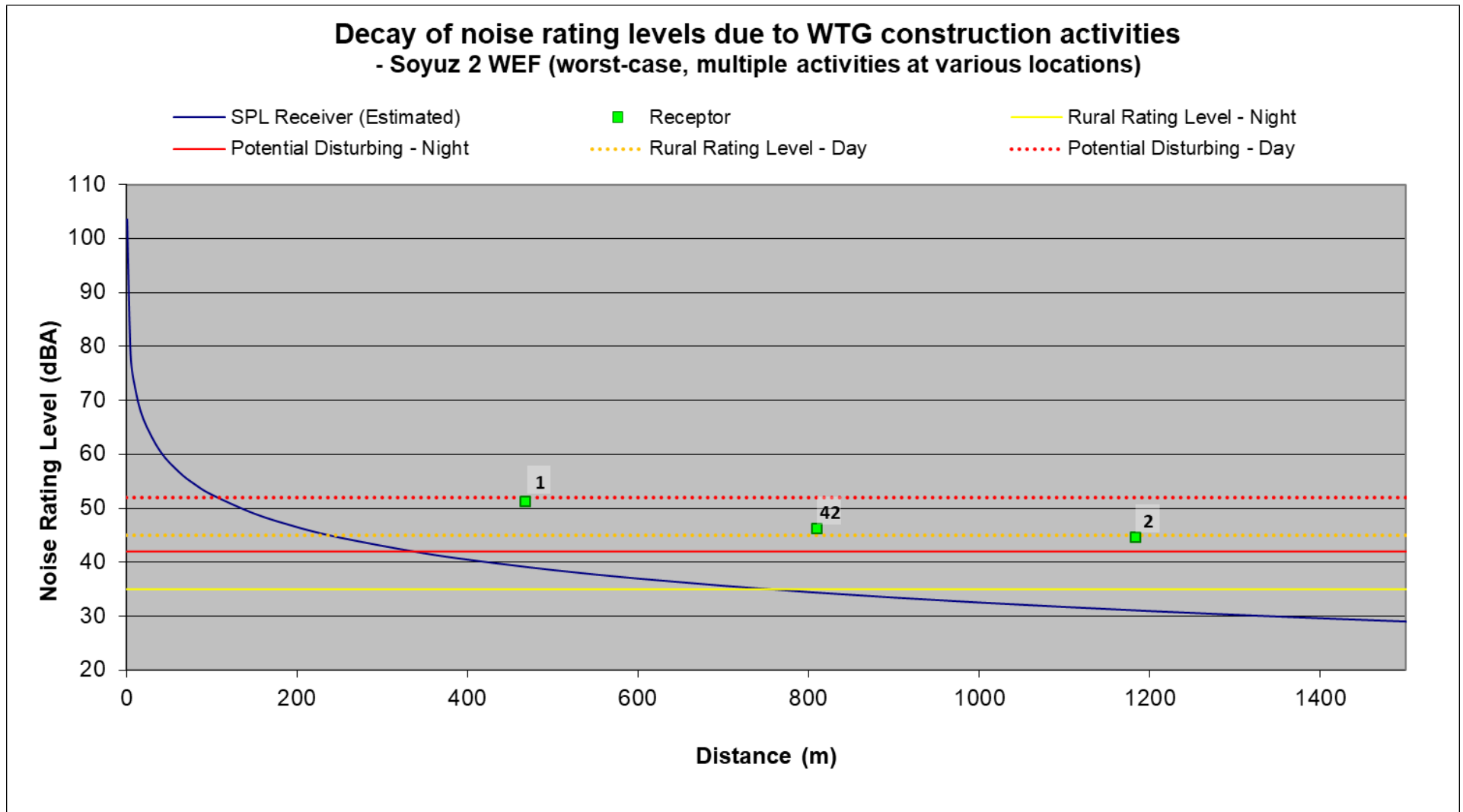
Figure 9-3: Projected conceptual construction noise levels for the proposed Soyuz 2 WEF
