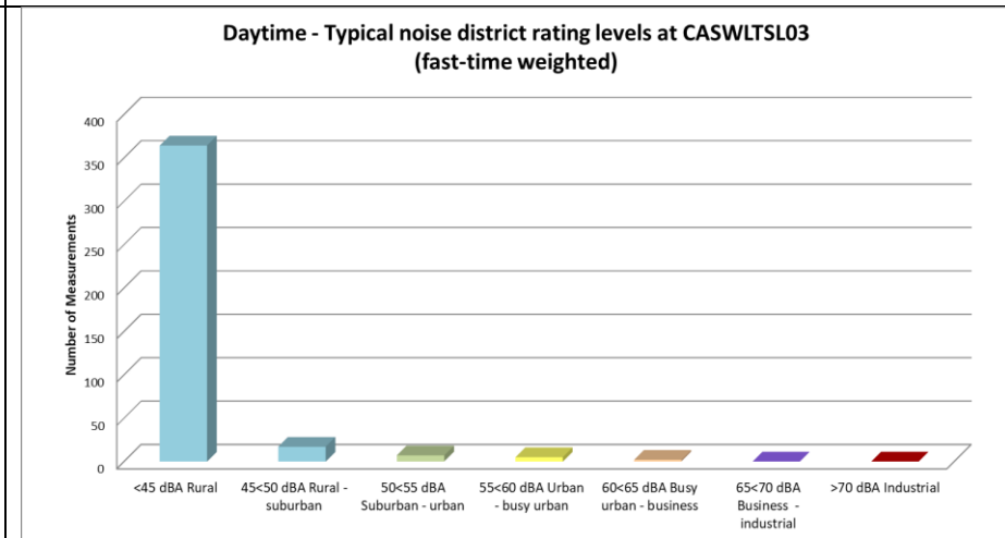
Figure 4-15: Classification of daytime measurements in typical noise districts at CASWLTSLO3
