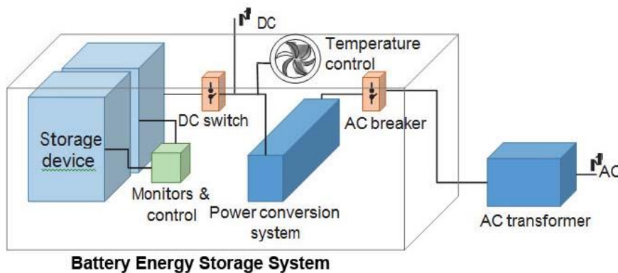
Figure 5-5: Conceptual BESS components 26
