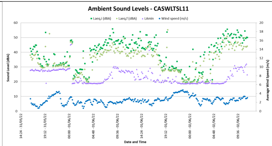
Figure 4-44: Ambient Sound Levels at CASWLTS11
