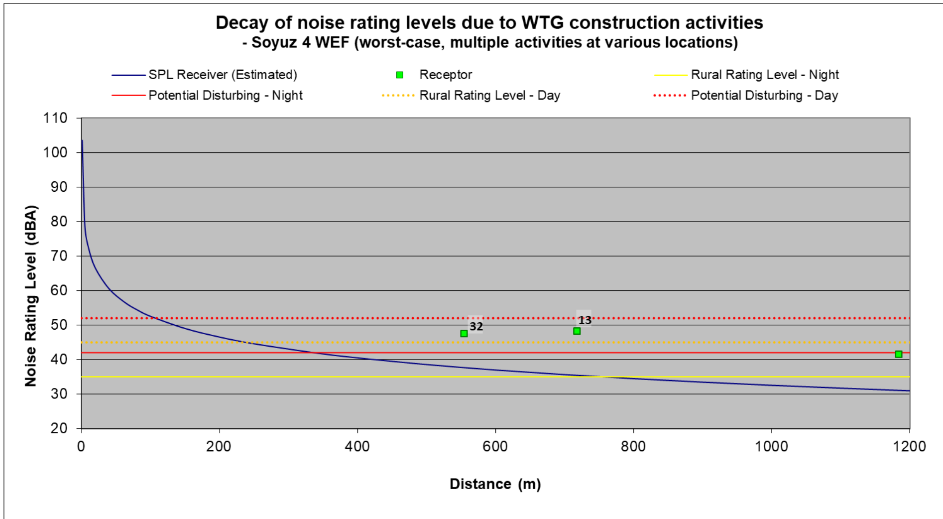
Figure 9-3: Projected conceptual construction noise levels for the proposed Soyuz 4 WEF
