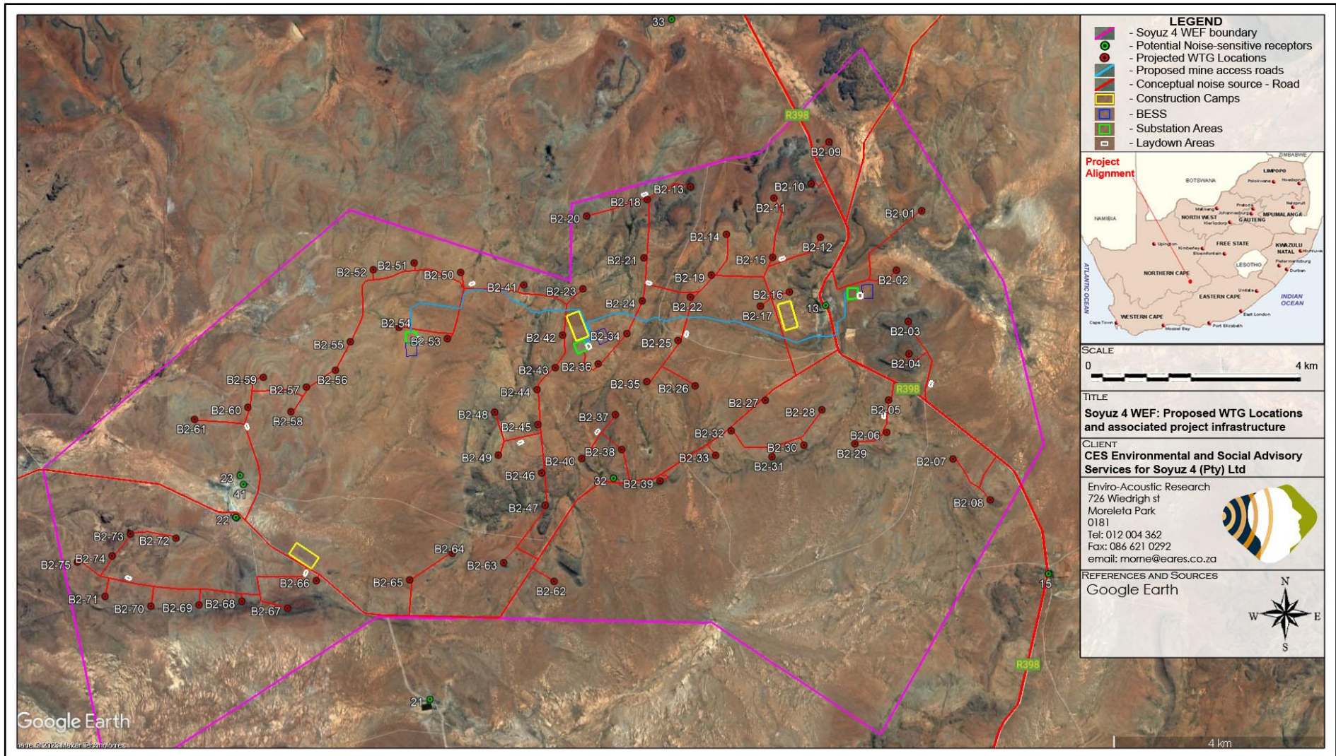
Figure 9-1: WTG locations and associated infrastructure for the proposed Soyuz 4 WEF
