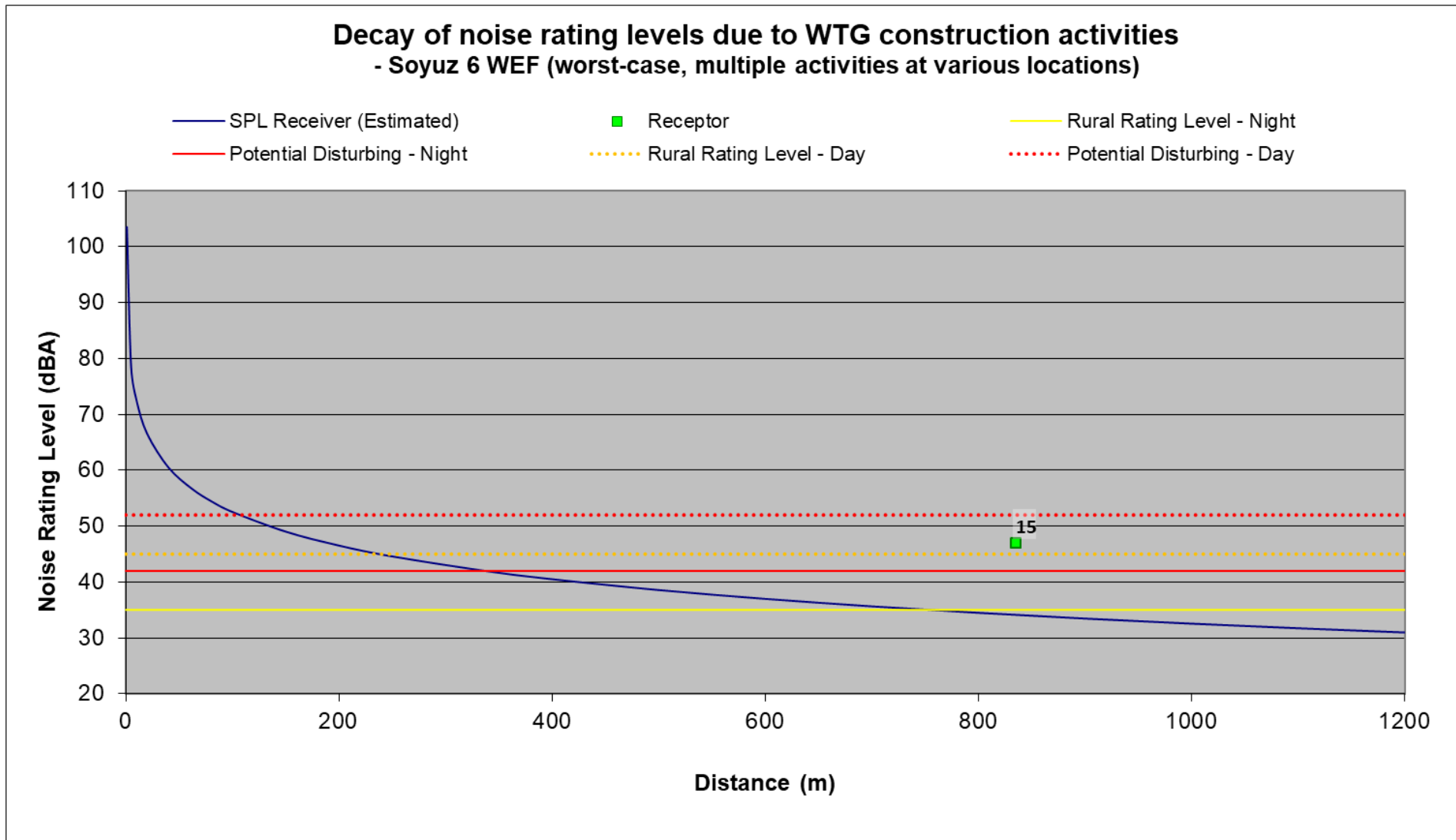
Figure 9-3: Projected conceptual construction noise levels for the proposed Soyuz 6 WEF
