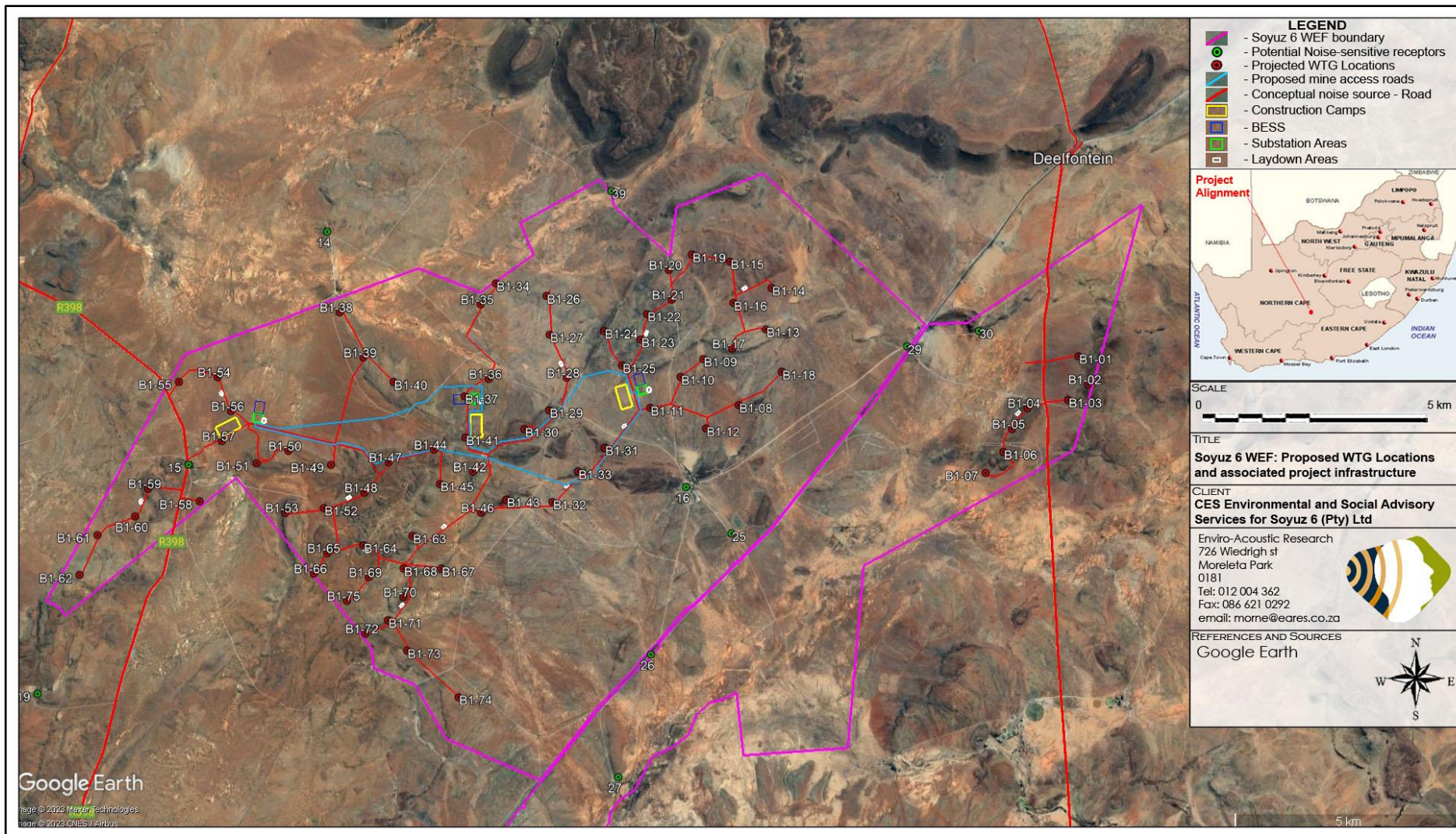
Figure 9-1: WTG locations and associated infrastructure for the proposed Soyuz 6 WEF
