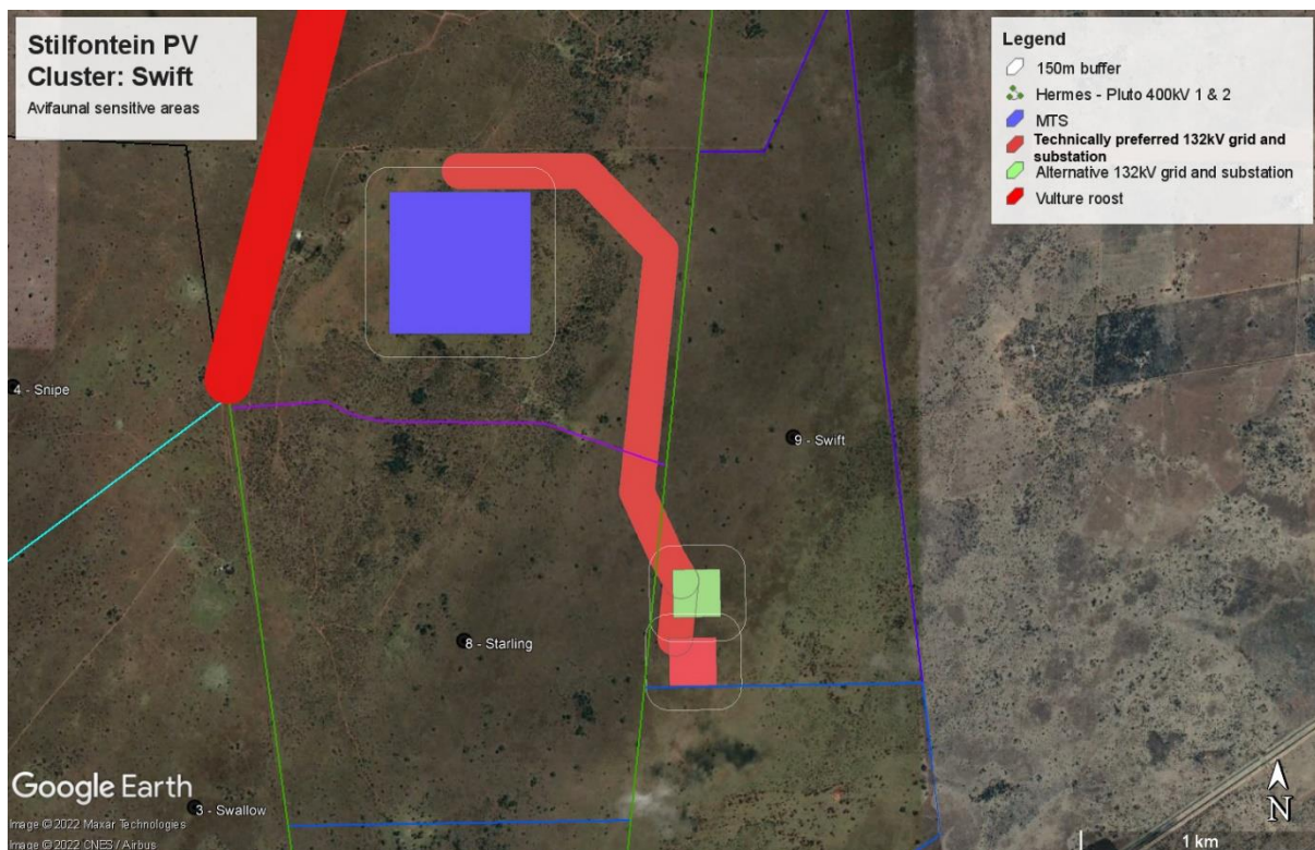
Figure D1: Swift grid sensitivities map
