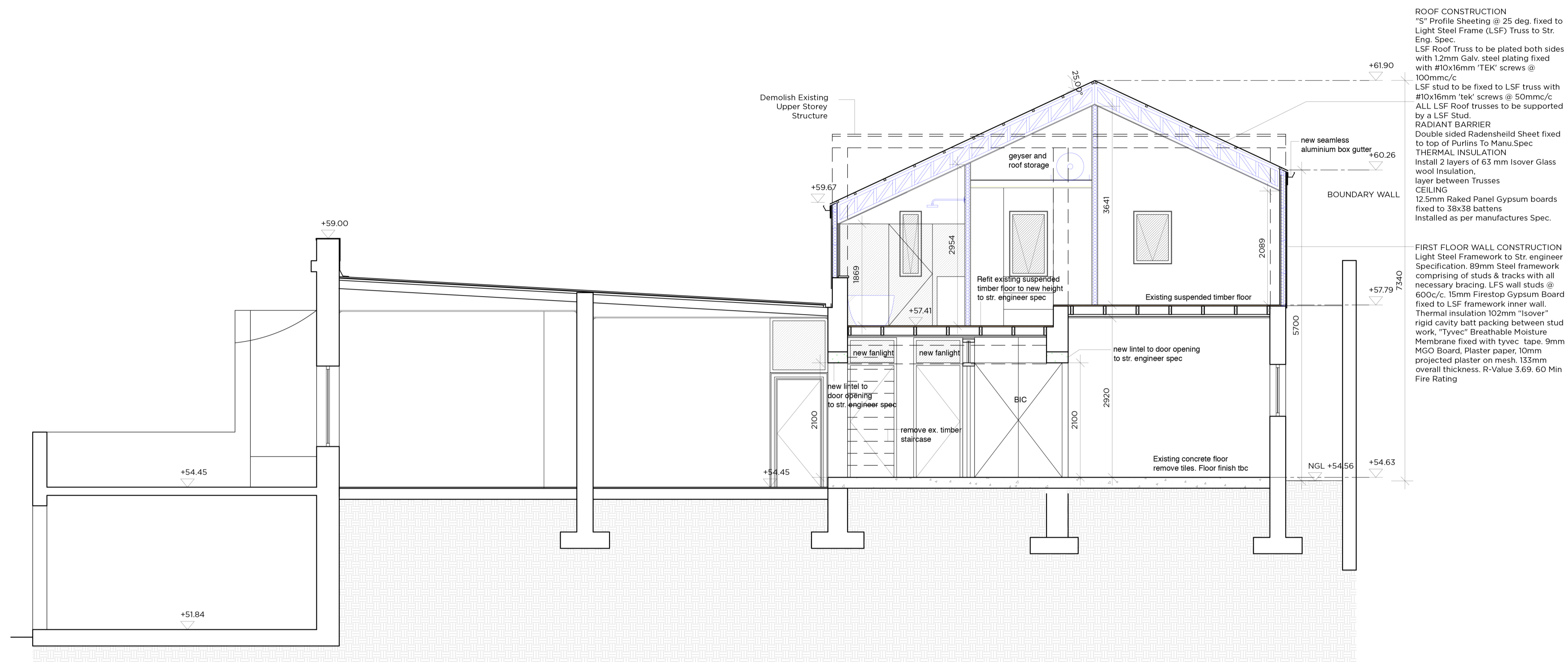
SECTION AA 1:50
