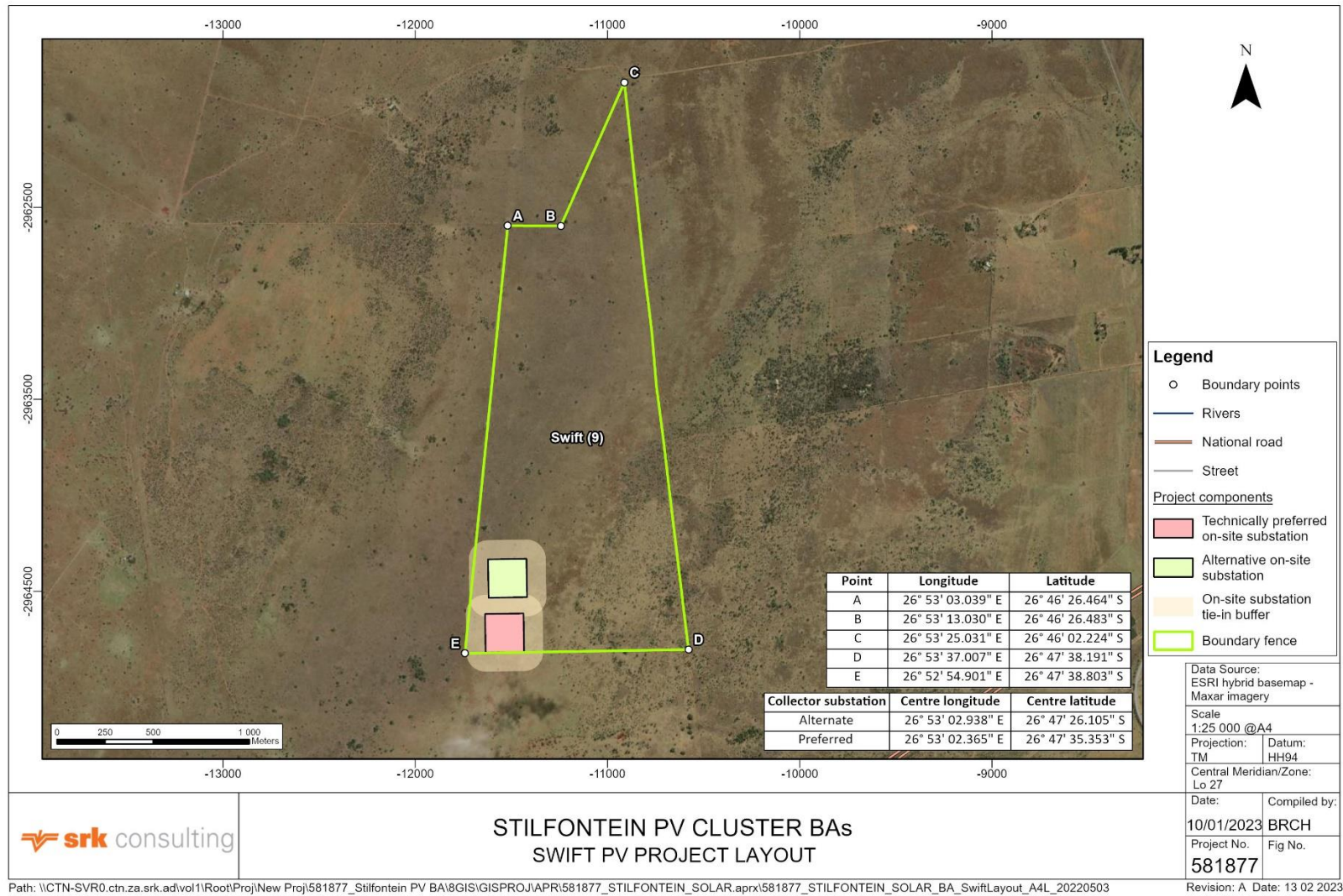
Figure 1-3: Layout of the Swift project
