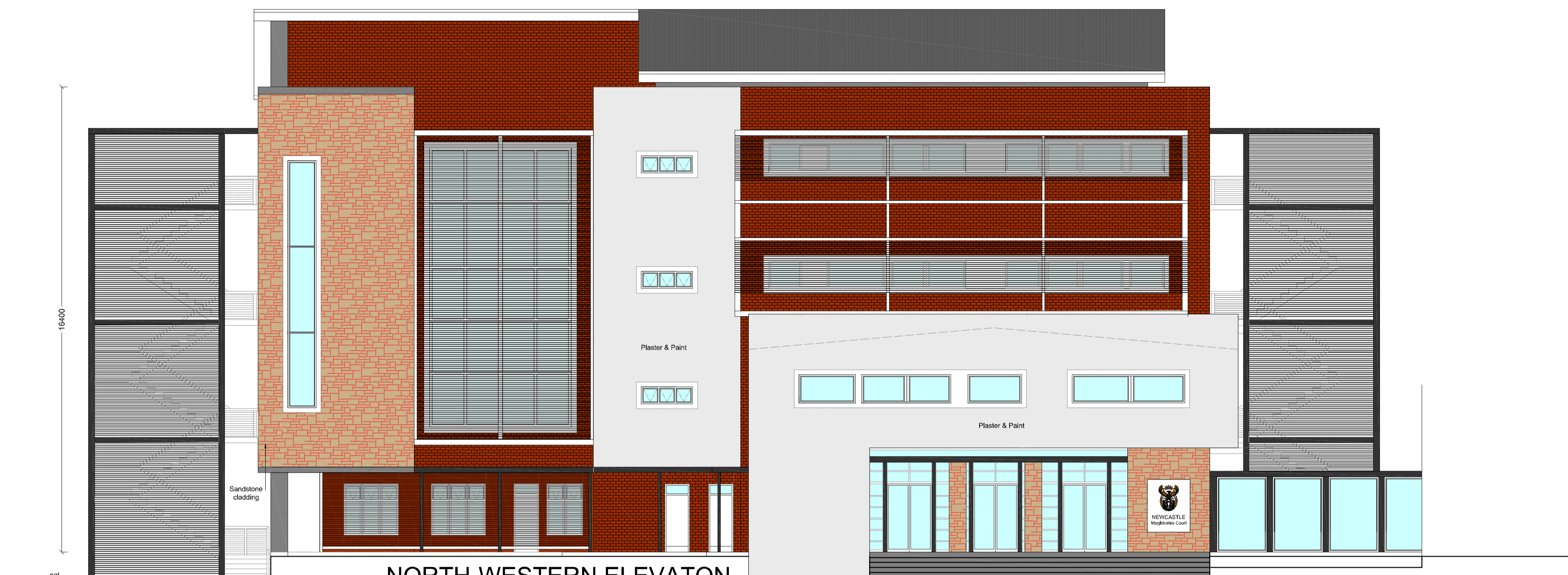
NORTH-WESTERN ELEVATION Scale 1:100
