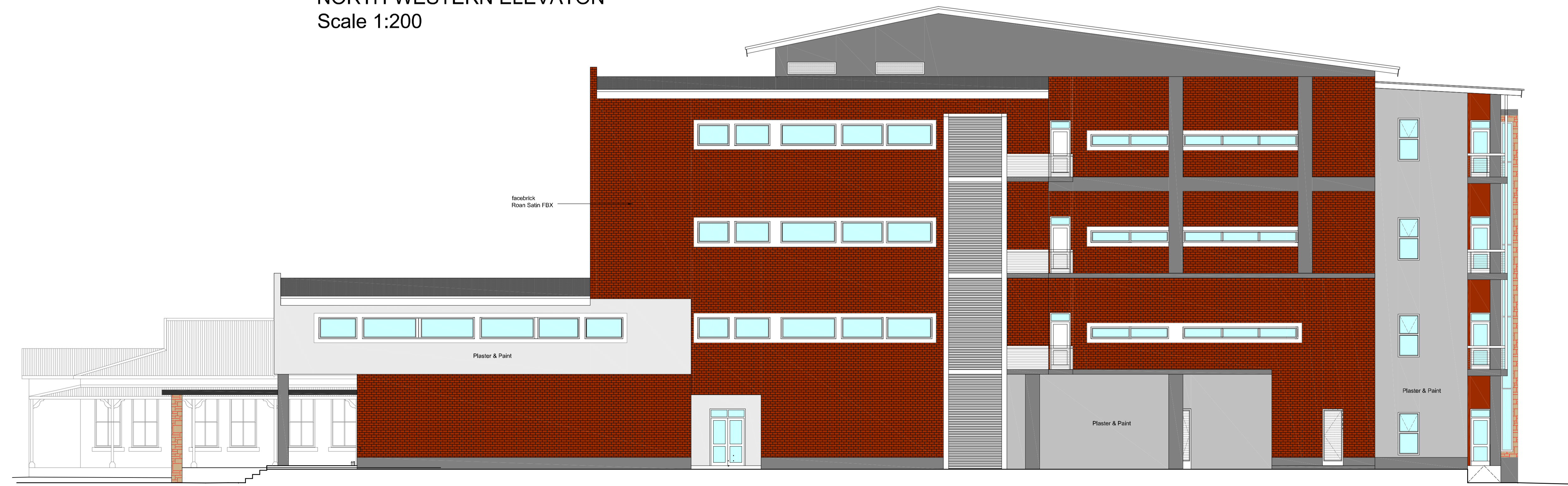
SOUTH WESTERN ELEVATION Scale 1:100
