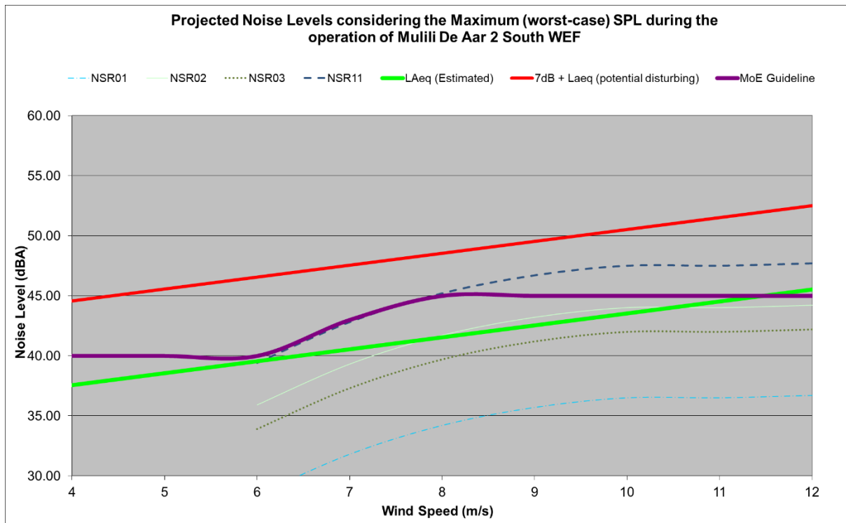
Figure 10-1: Projected noise levels at different wind speeds considering the worst-case SPL of the Goldwind GW165-6.0 WTG
