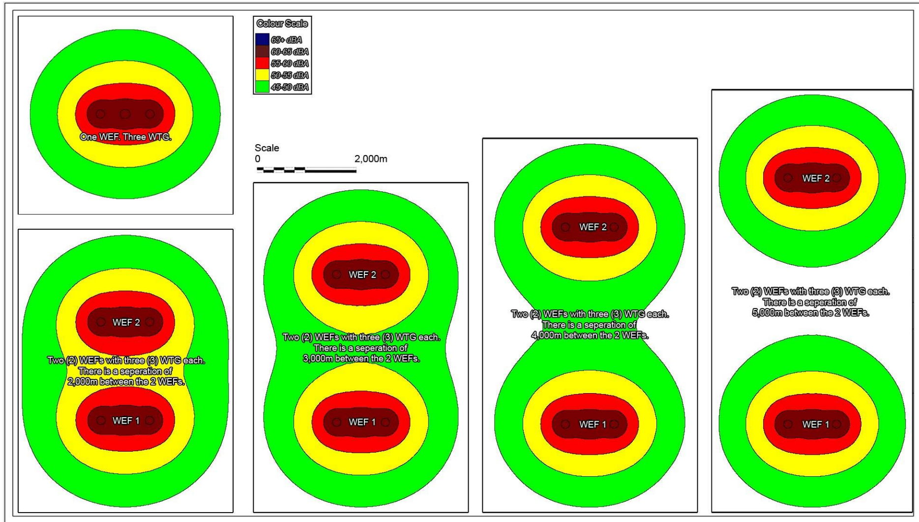
Figure 9-2: Effect of distance between wind turbines – potential cumulative noise
