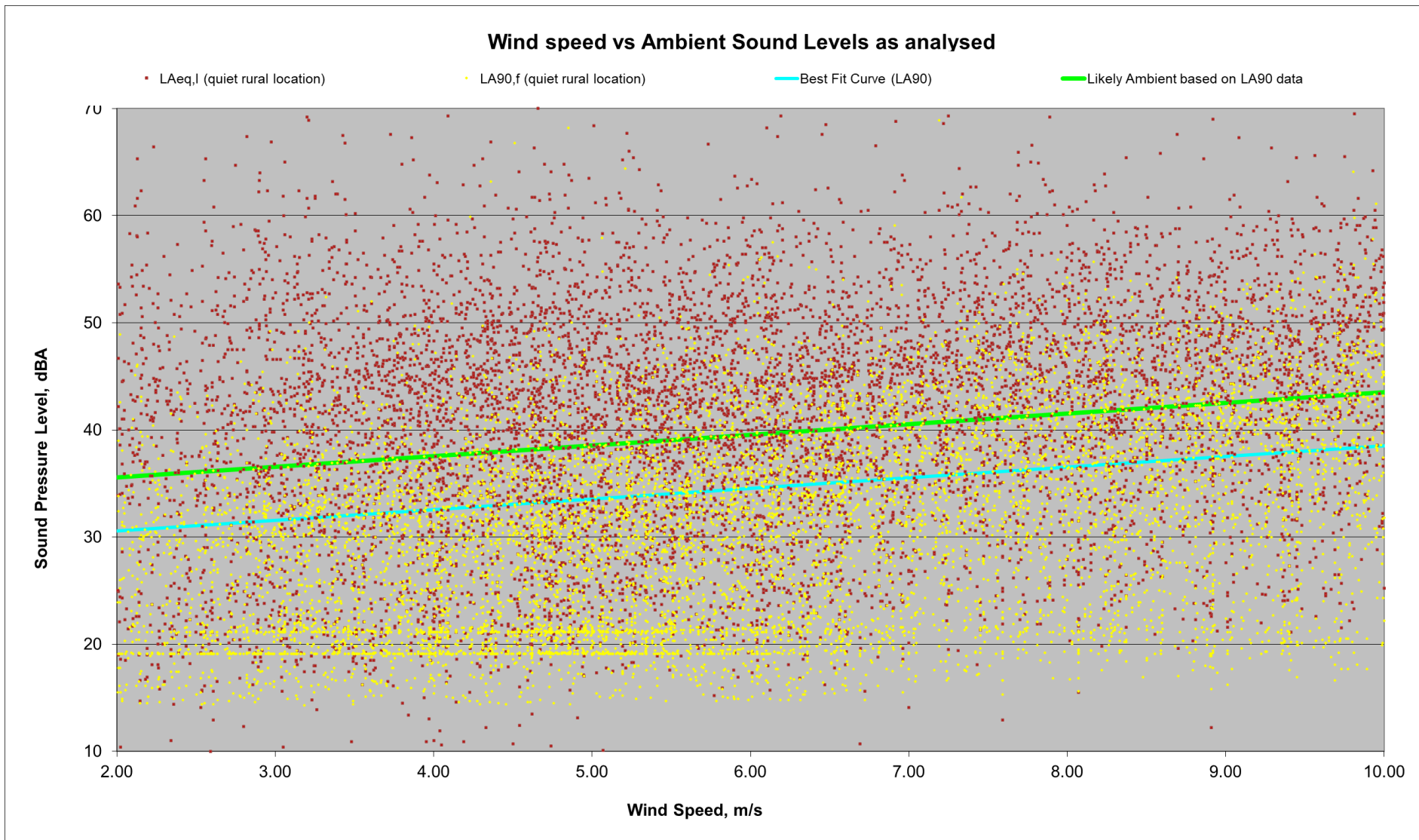
Figure 4-2: Result of regression analysis of ambient sound levels measured in Karoo area
