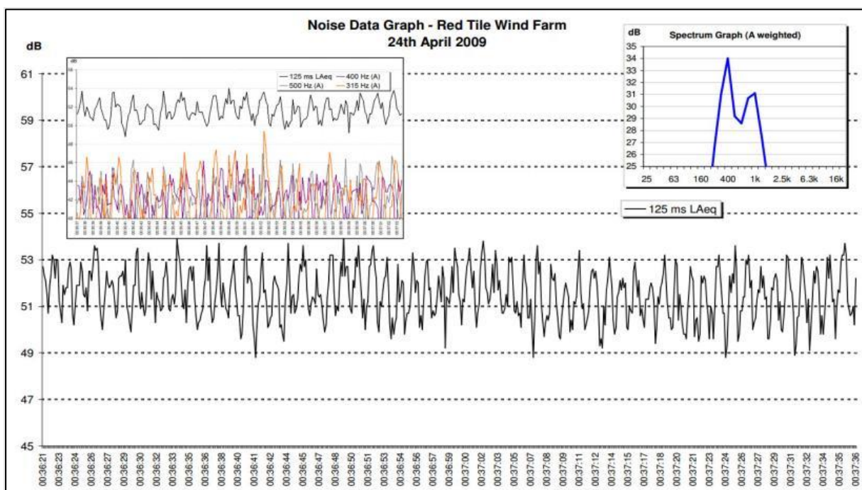
Figure 5-4: Example time-sound series graph illustrating AM as measured by Stigwood (2013) [122]
