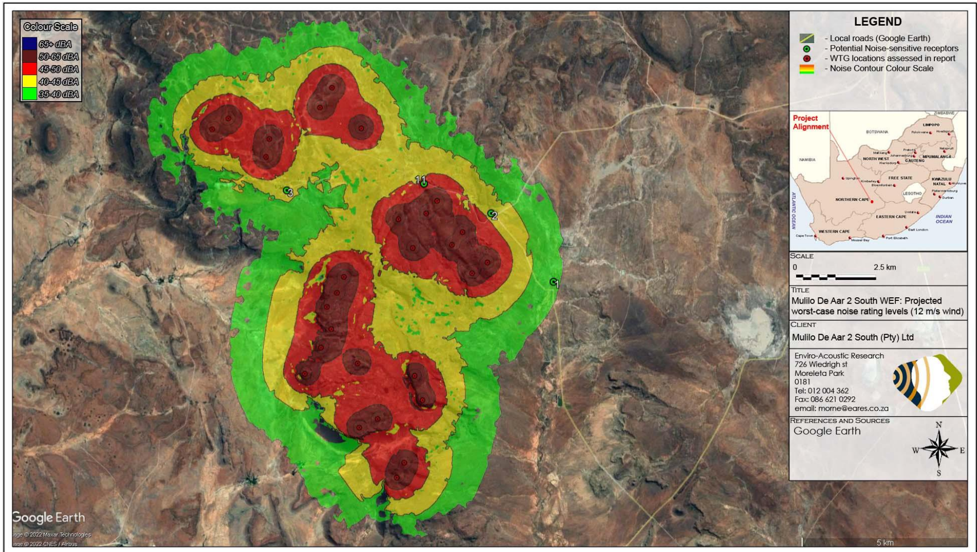
Figure 9-1: Projected future noise rating level contours (worst-case SPL of 112.6 dBA re 1 pW)
