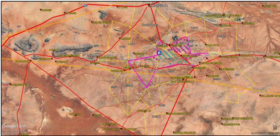
Figure 3.3: De Rust North site properties (pink outline) in relation to adjacent properties (yellow outlines), proposed turbines (pink circles), proposed construction and operational premises (dark blue circle), proposed access points 1-5 (white triangles). Also indicated are proposed South WEF turbines (blue circles), existing transmission lines (orange), and the study area road network (red)
