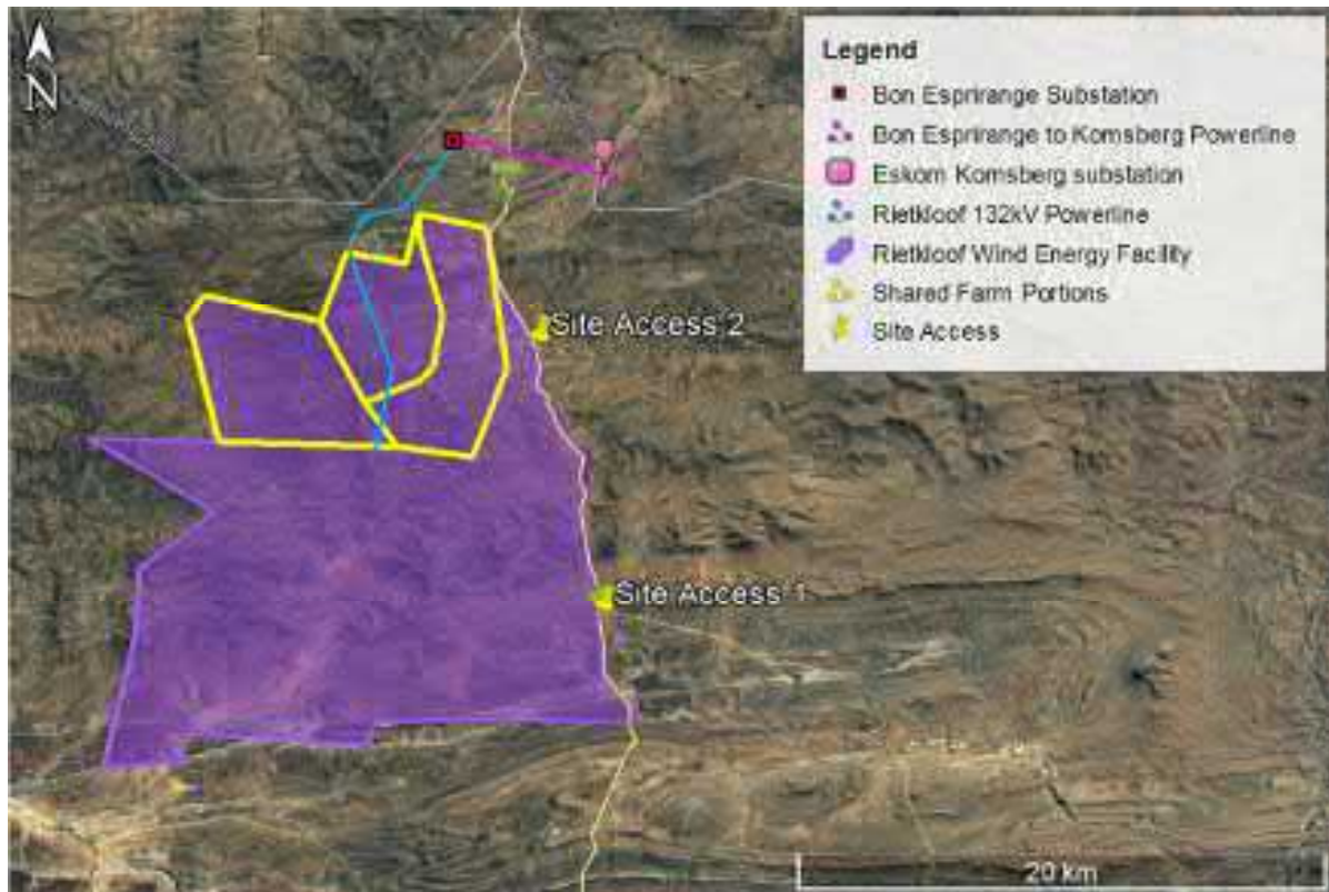
Figure 2-2: 132 KV Powerline
