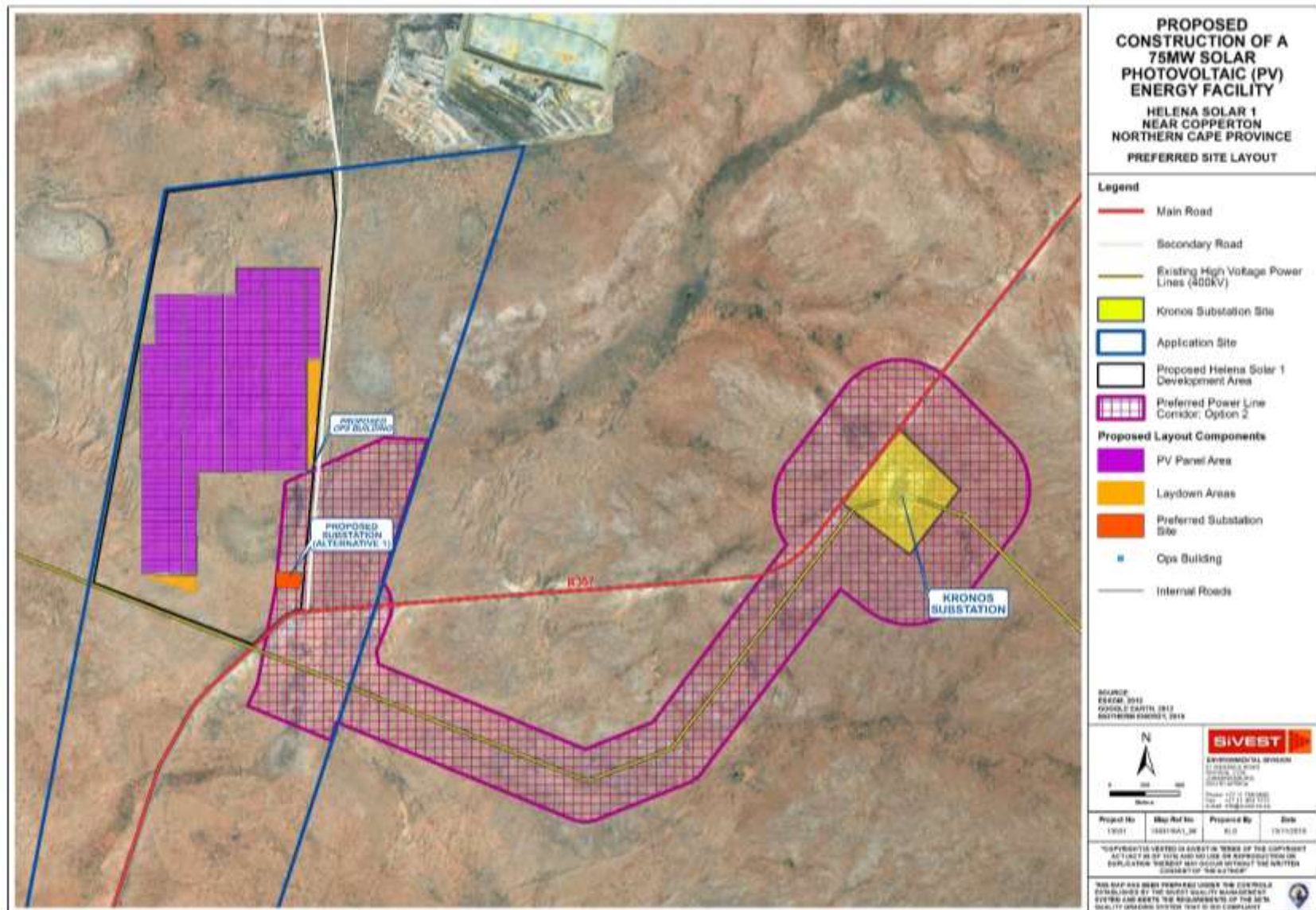
Figure 81: Preferred Site Layout
