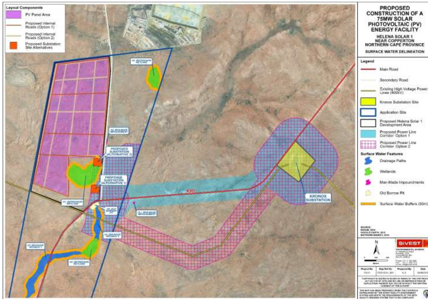
Figure 32. In-field delineated Surface Water Resources within the Helena 1 Proposed Development Site
