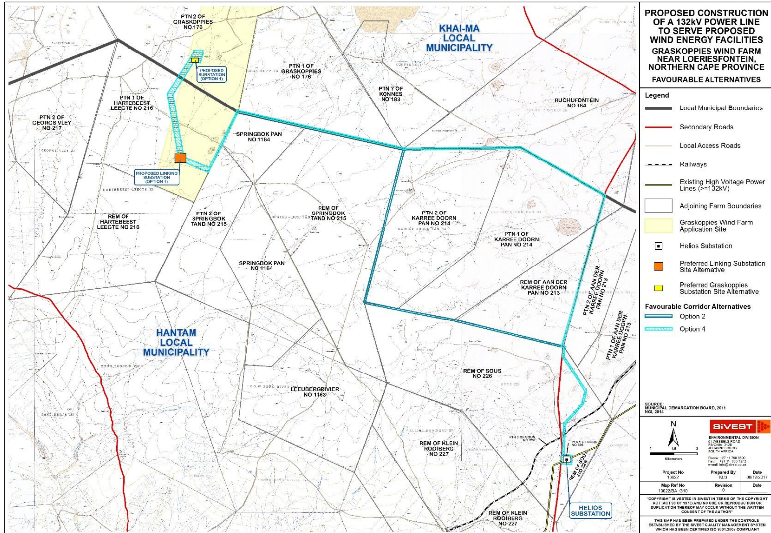
Figure iv: Preferred Graskoppies On-site Eskom Substation, Linking Substation and Favourable Power Line Corridor Alternatives
