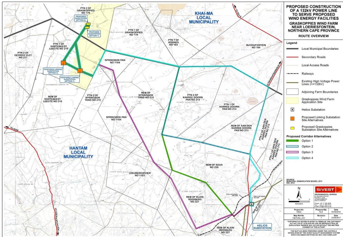
Figure 1: Route overview for the proposed Graskoppies On-site Eskom Substation, 132kV Linking Substation and associated 132kV power line
