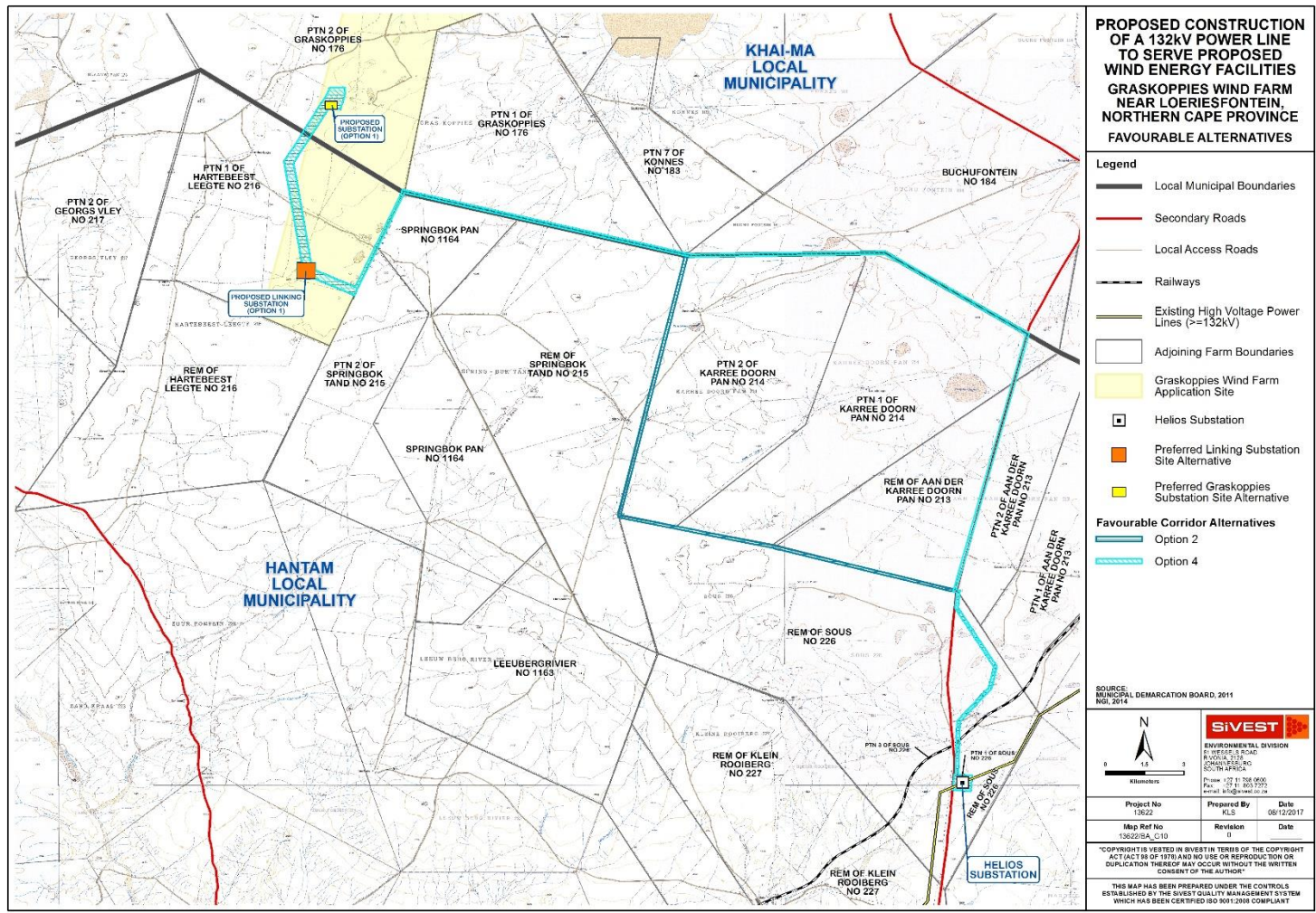
Figure 71: Preferred substation site and favourable power line corridor alternatives
