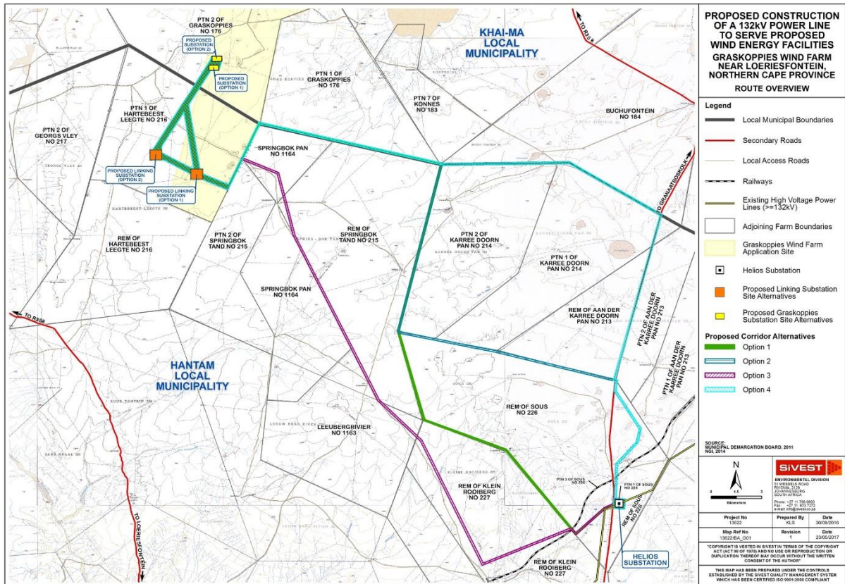
Figure 9: Power Line Route Overview, including all alternatives
