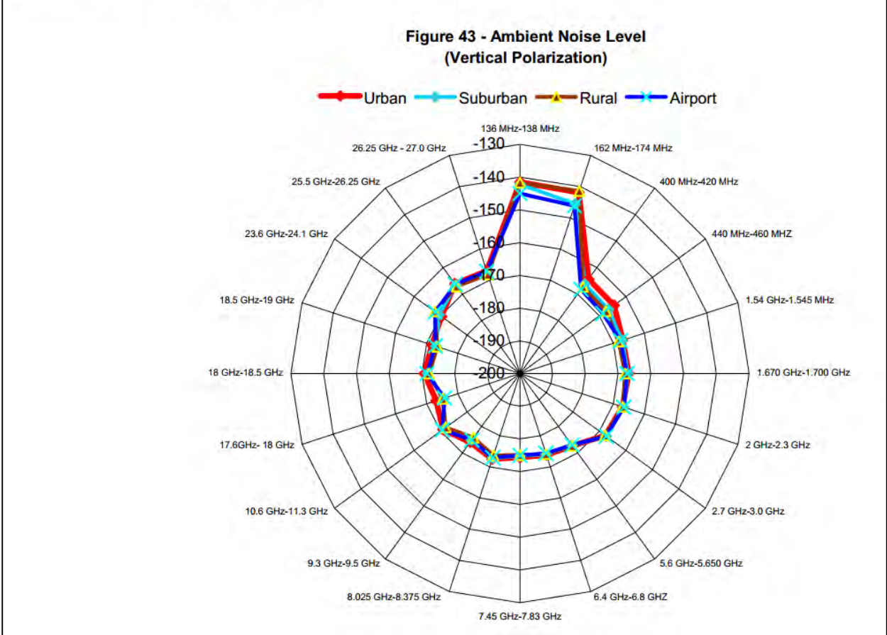
Figure 155: Measured ambient data comparison – Vertical polarization
