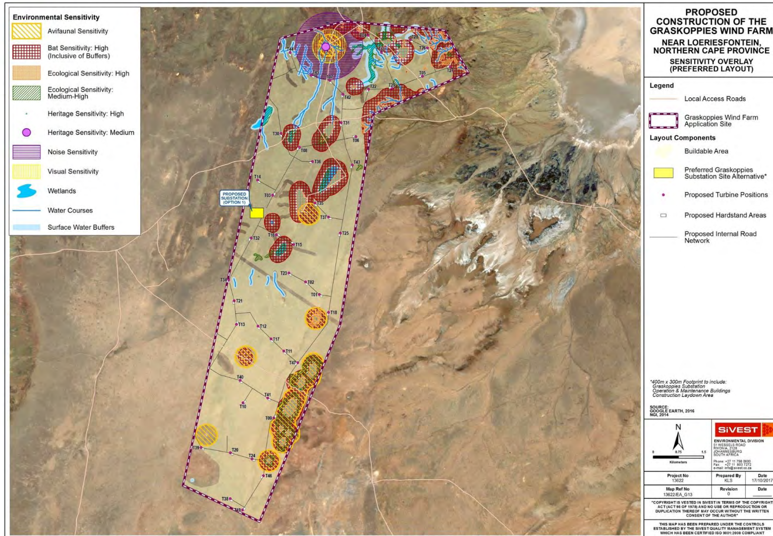
Figure vi: Preferred Graskoppies 47 Turbine Layout showing Environmentally Sensitive Areas
