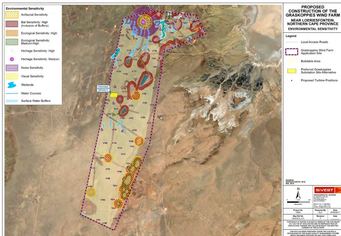
Figure 157: Proposed Graskoppies 70 Turbine Layout Alternatives and EIA Phase Environmental Sensitivity
