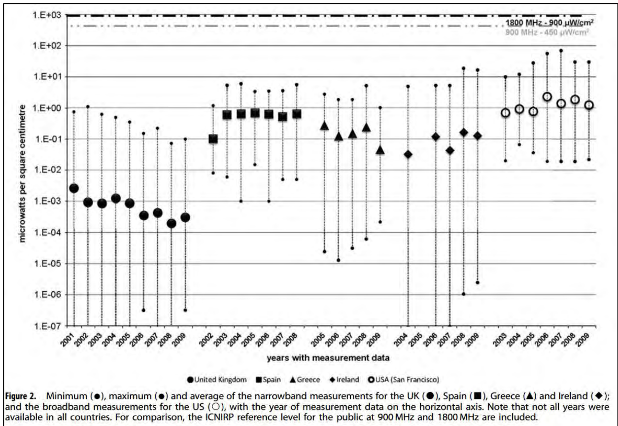
Figure 156: Comparison of ambient data for different years in different countries
