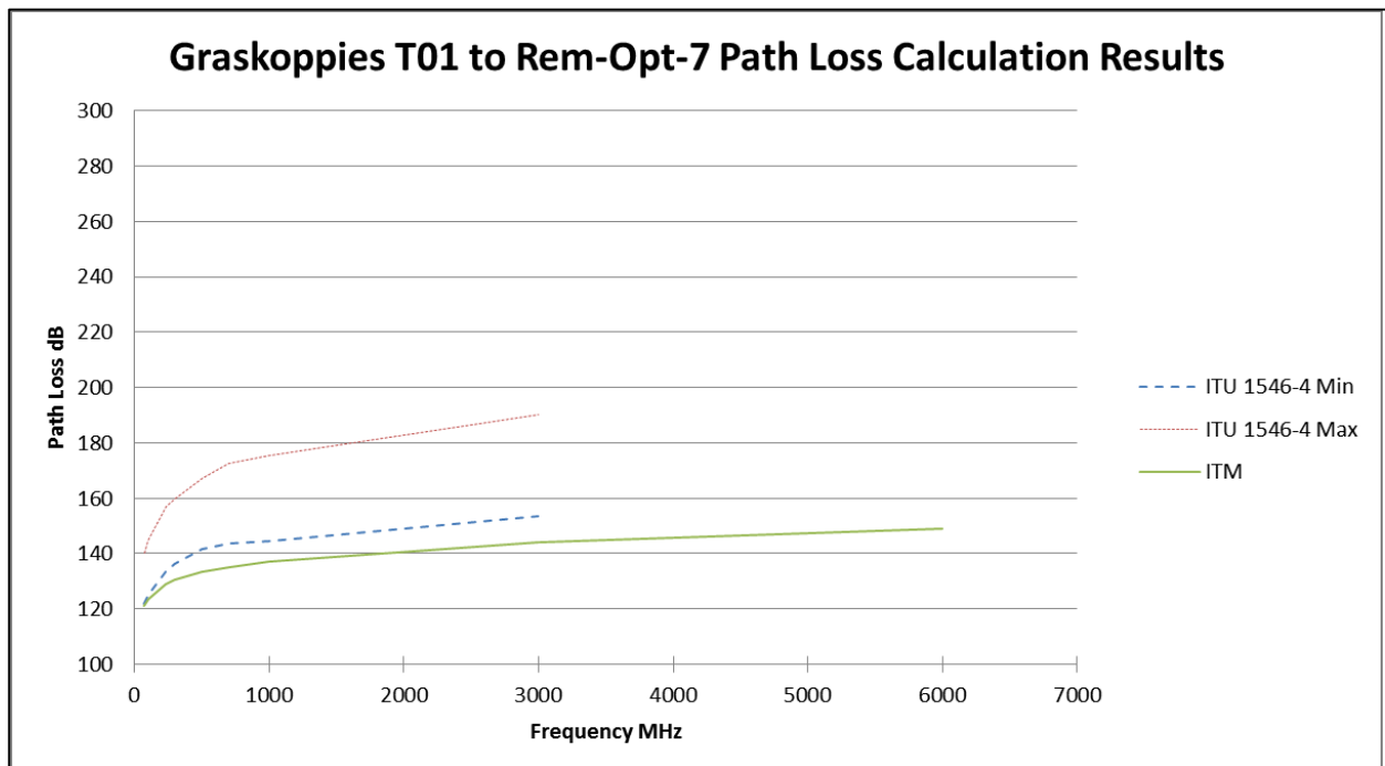
Figure 145: WTG 1 (150m height) to SKA Rem Opt 7 Path Loss Calculation result
