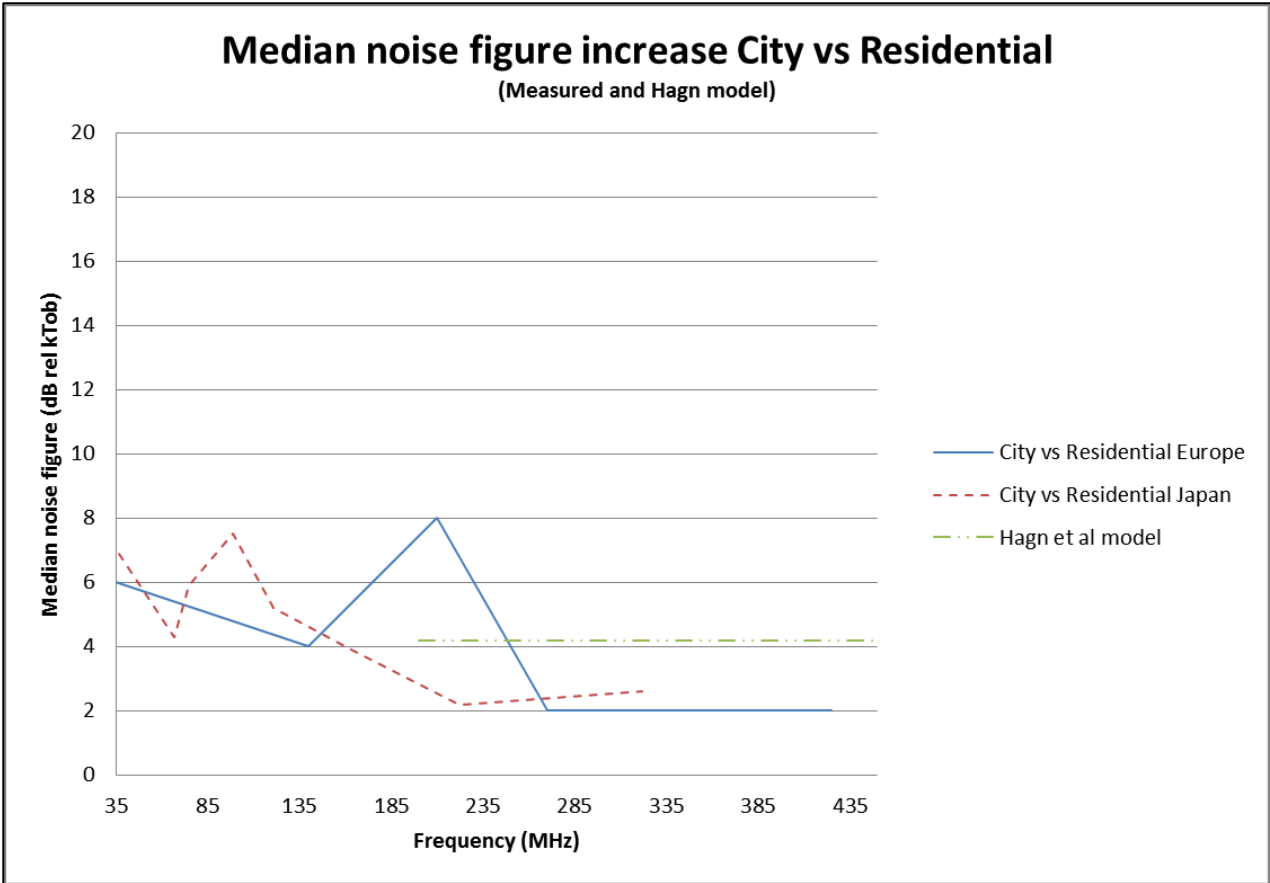
Figure 153: Man-made noise measured results (ITU-R P.372-13 Table 3 and Table 4, Hagn eq 8 and 9)
