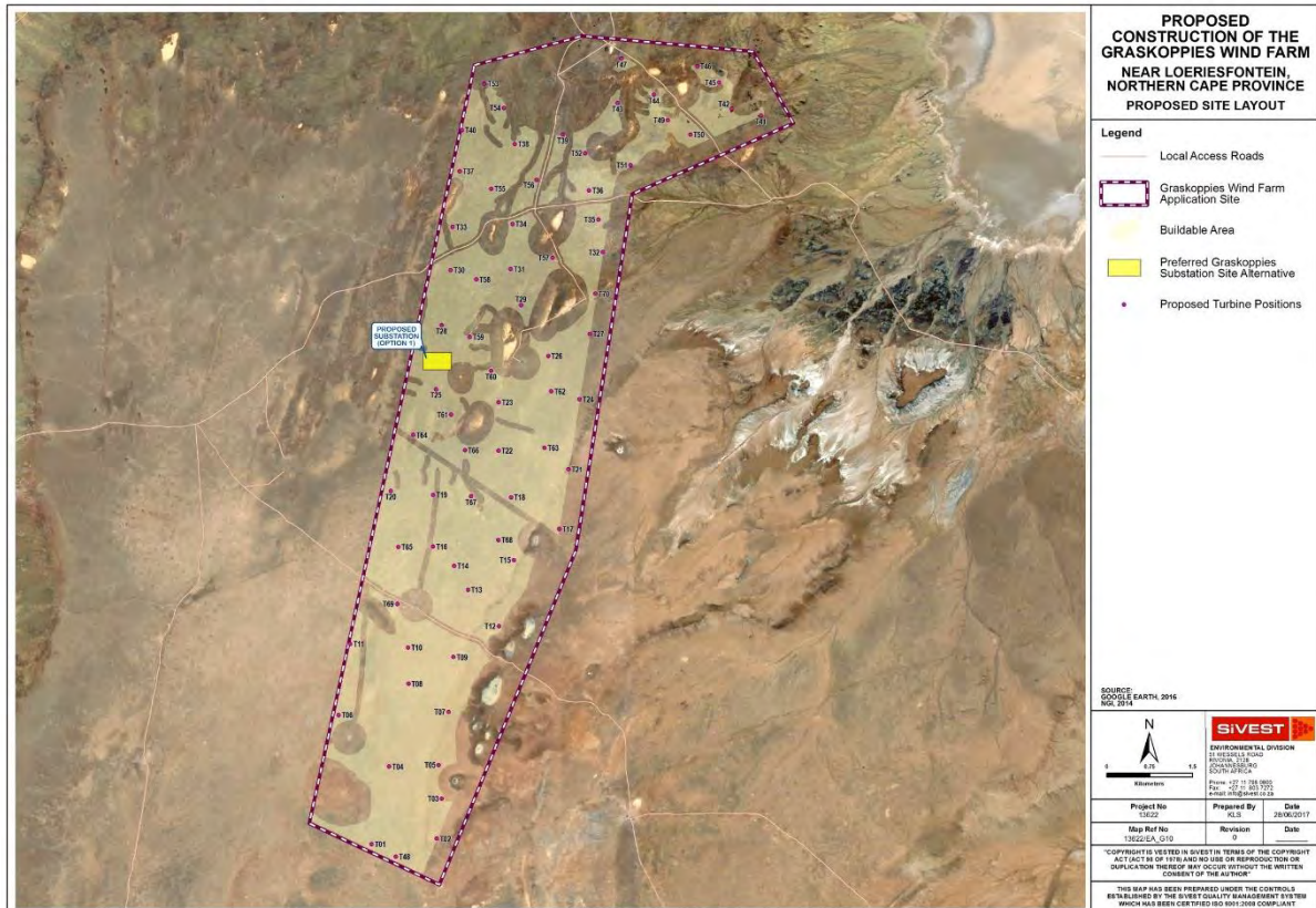
Figure 4: Proposed Preferred Graskoppies Layout
