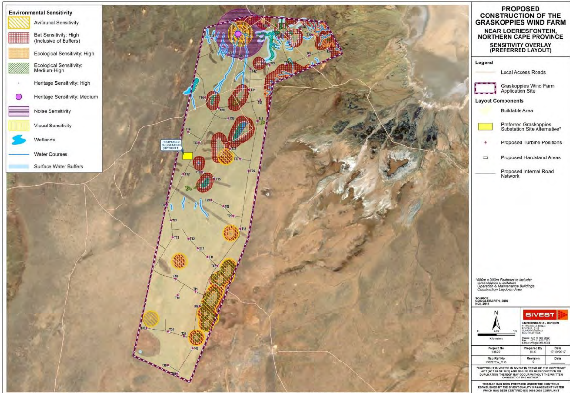
Figure 158: Proposed EIA Phase 47 wind turbine layout alternatives in relation to sensitive areas
