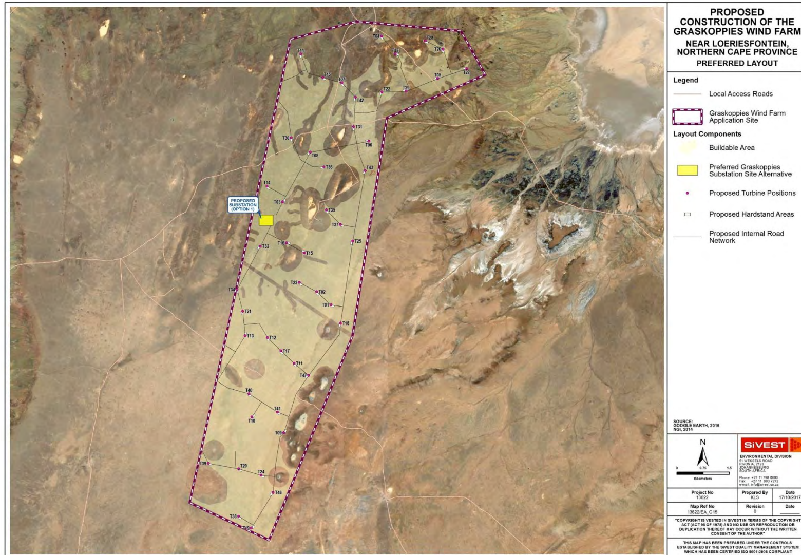
Figure v: Preferred Graskoppies 47 Turbine Layout
