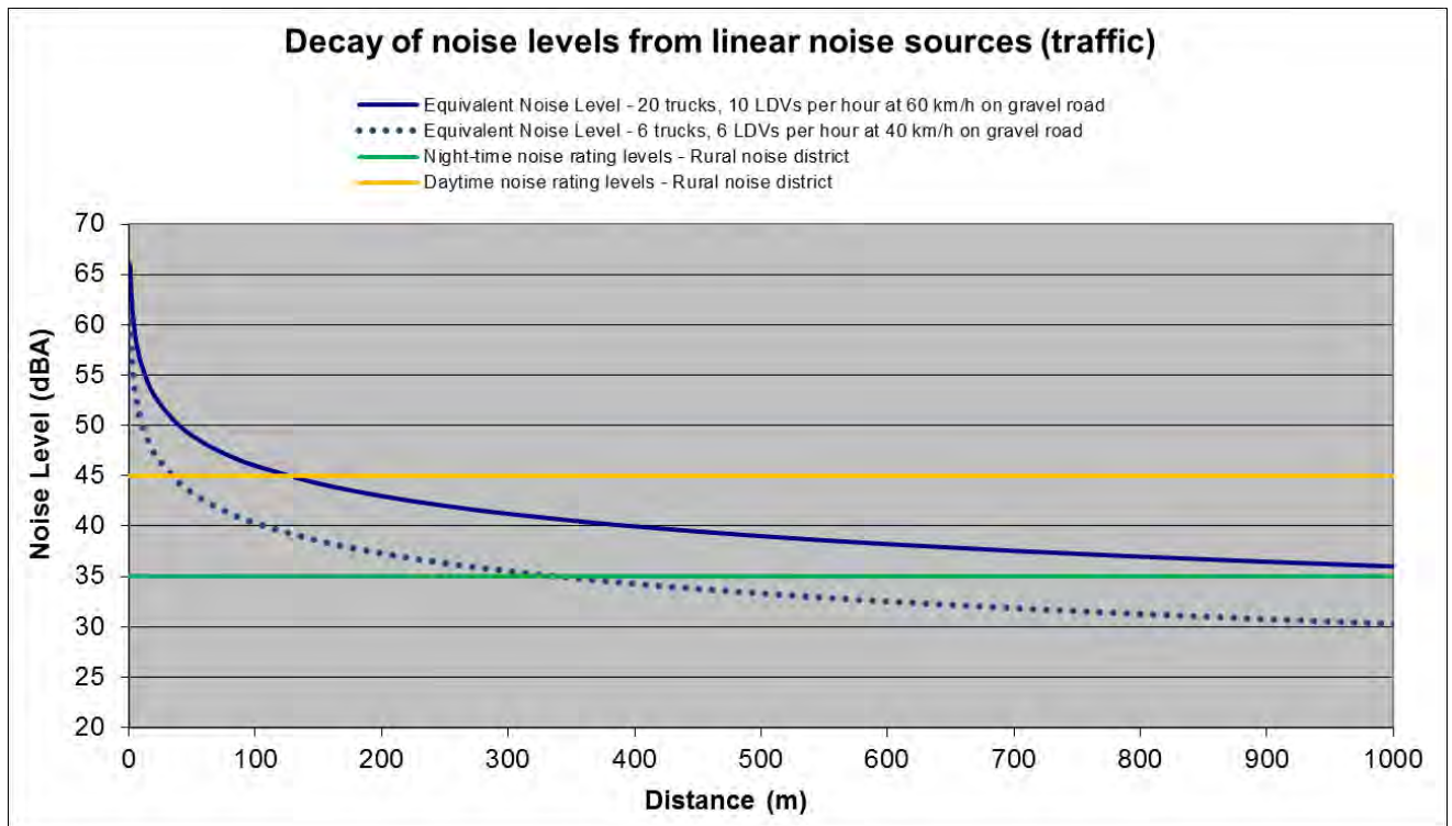
Figure 98: Projected conceptual construction traffic noise levels – Decay over distance from linear activities
