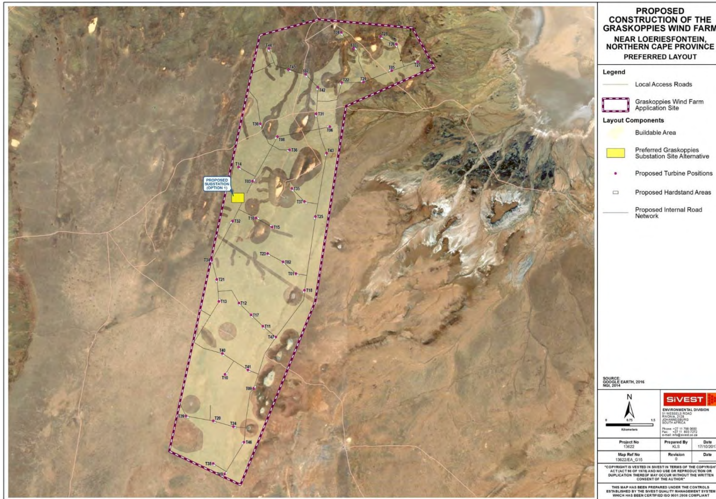
Figure 160: Preferred Graskoppies 47 Turbine Site Layout
