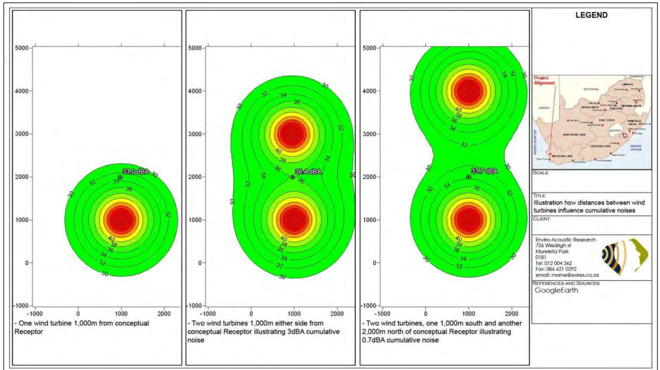
Figure 149: Effect of distance between wind turbines – potential cumulative noise levels
