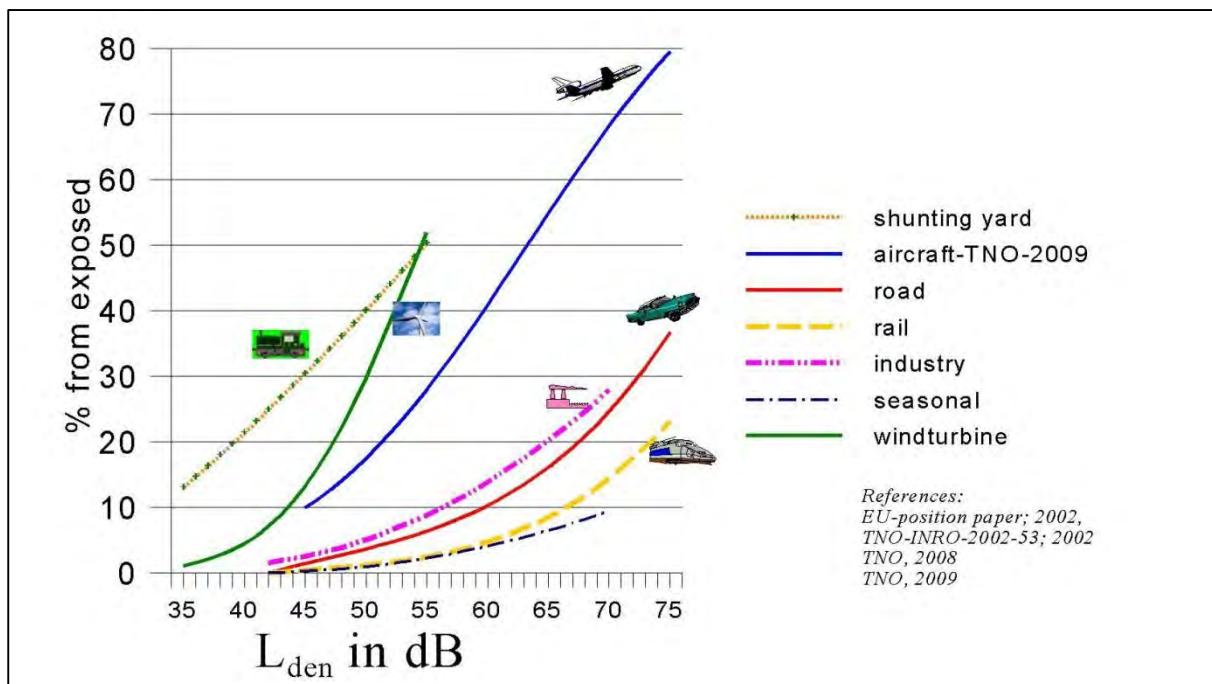
Figure 96: Percentage of annoyed persons as a function of the day-evening-night noise exposure at the façade of a dwelling
