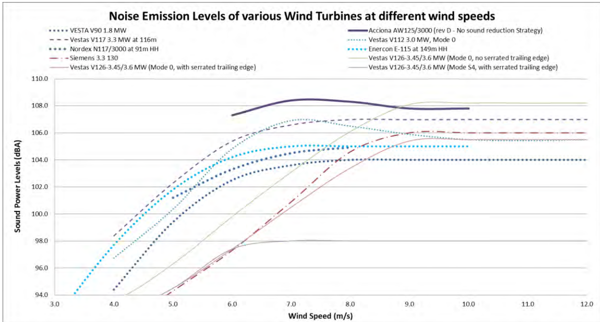
Figure 93: Noise Emissions Curve of a number of different wind turbines
