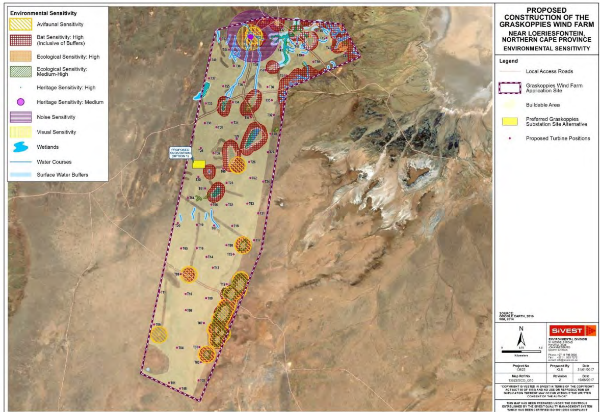
Figure 7: Proposed Graskoppies 70 Turbine Layout Alternatives and Scoping Phase Environmental Sensitivity
