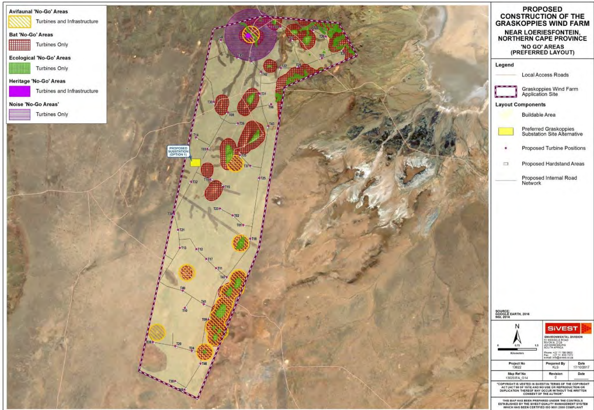
Figure 159: Proposed EIA Phase 47 turbine layout alternatives in relation to no-go areas
