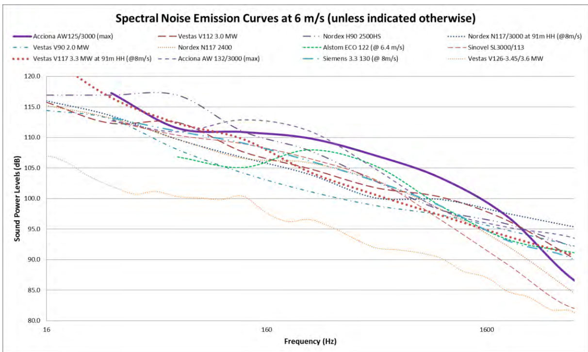
Figure 94: Octave sound power emissions of various wind turbines
