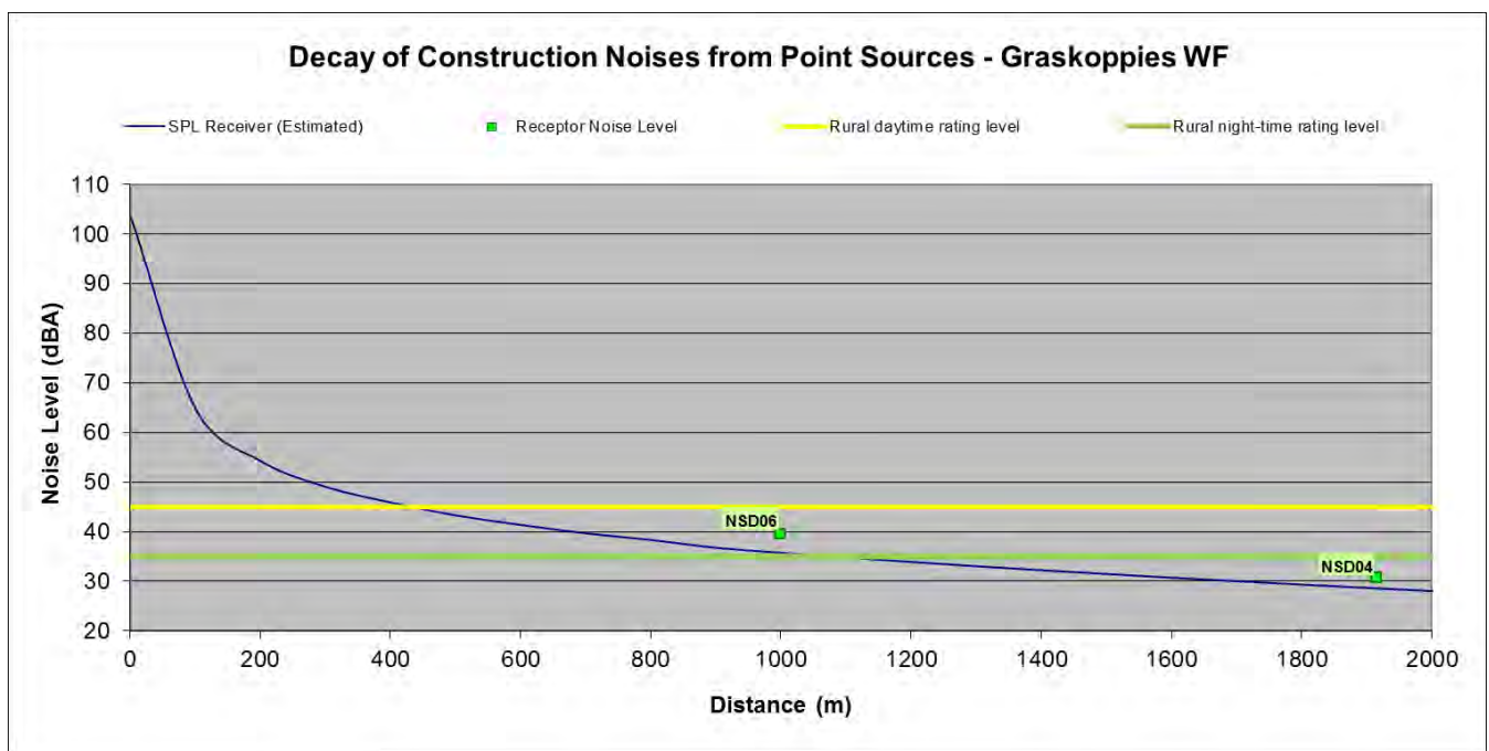
Figure 97: Projected conceptual construction noise levels – Decay of noise from construction activities
