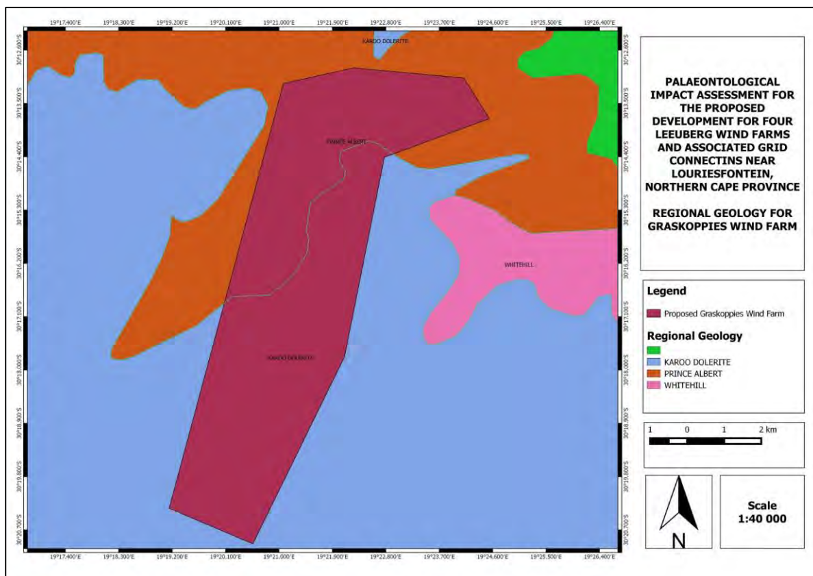
Figure 35: The surface geology of the proposed Graskoppies Wind Farm near Loeriesfontein in the Northern Cape Province. The development footprint is underlain by Karoo Dolerite as well as the Prince Albert and Whitehill Formations of the Ecca Group.
