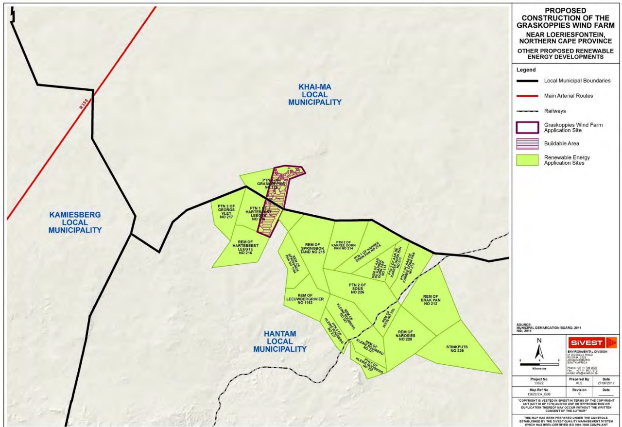
Figure 147: Location of the renewable energy developments proposed within a 55km radius of the proposed Graskoppies Wind Farm application site
