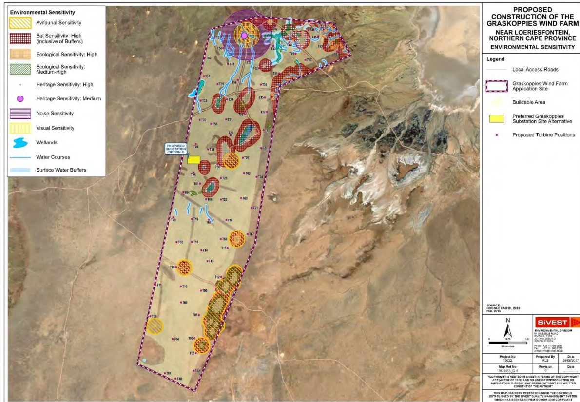
Figure iv: Graskoppies Wind Farm EIA Phase Layout Alternatives in relation to Environmental Sensitive Areas
