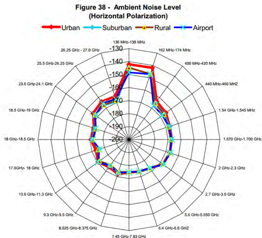
Figure 154: Measured ambient data comparison – Horizontal polarization
