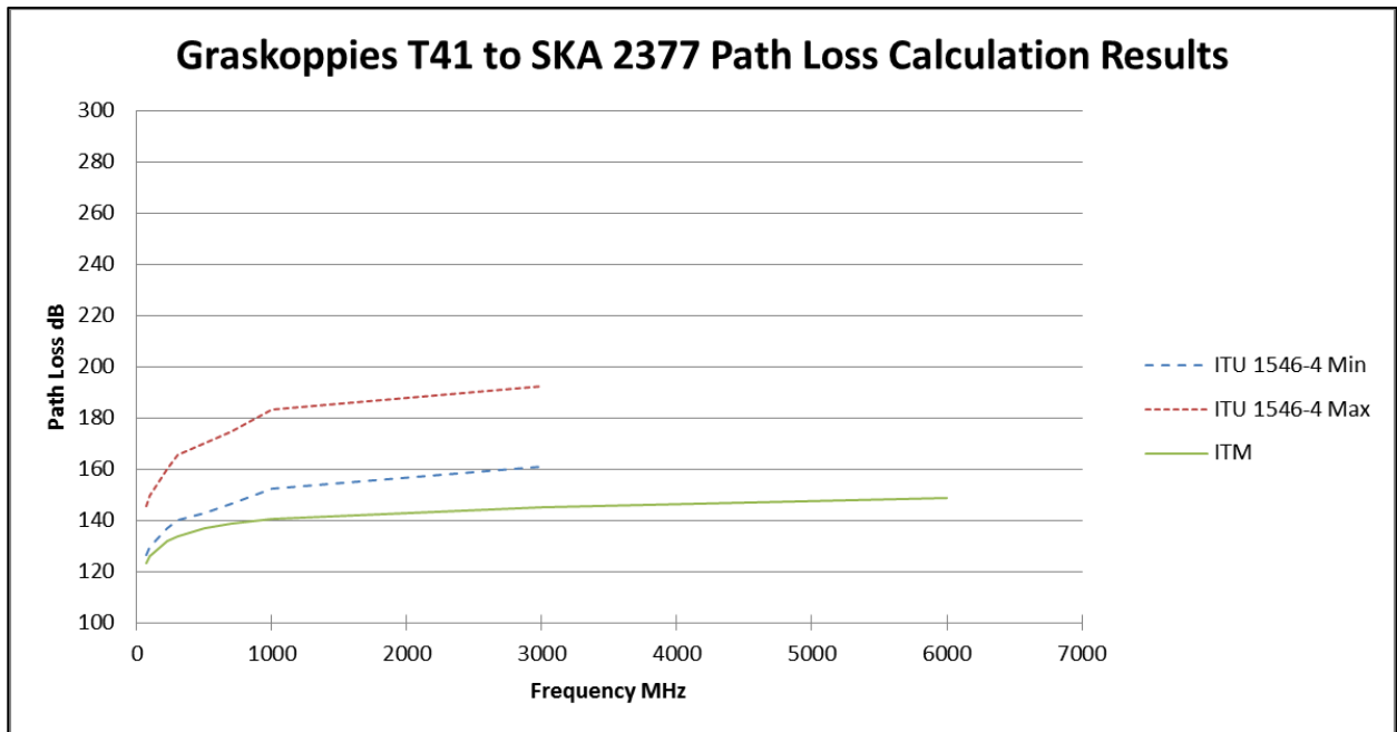
Figure 146: WTG 41 (150m) to SKA 2377 Path Loss Calculation result
