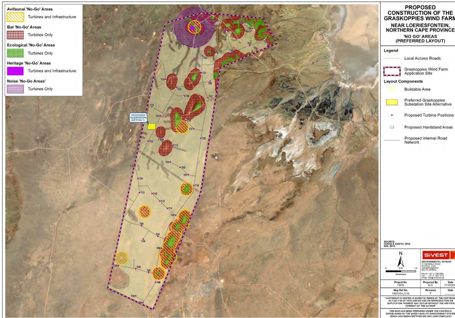
Figure 162: Preferred 47 Turbine Site Layout in relation to No-go Areas
