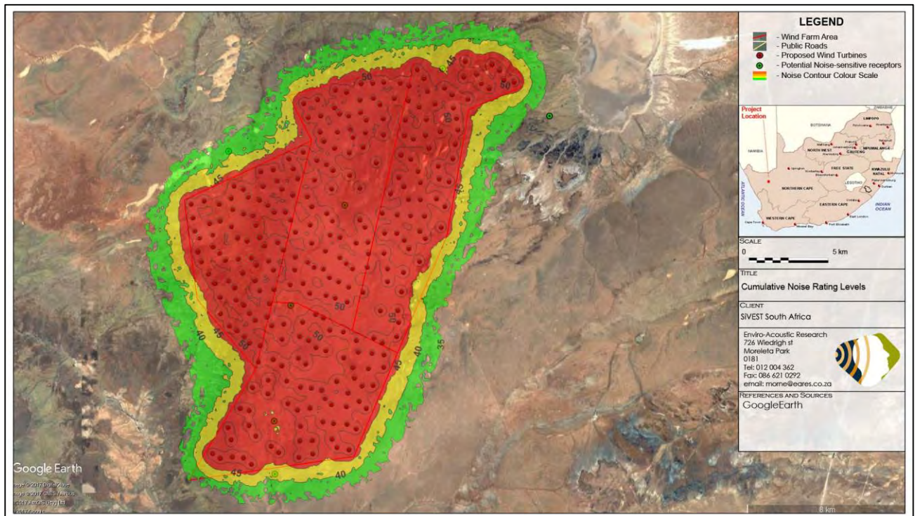
Figure 148: Projected conceptual cumulative noise rating levels during operation
