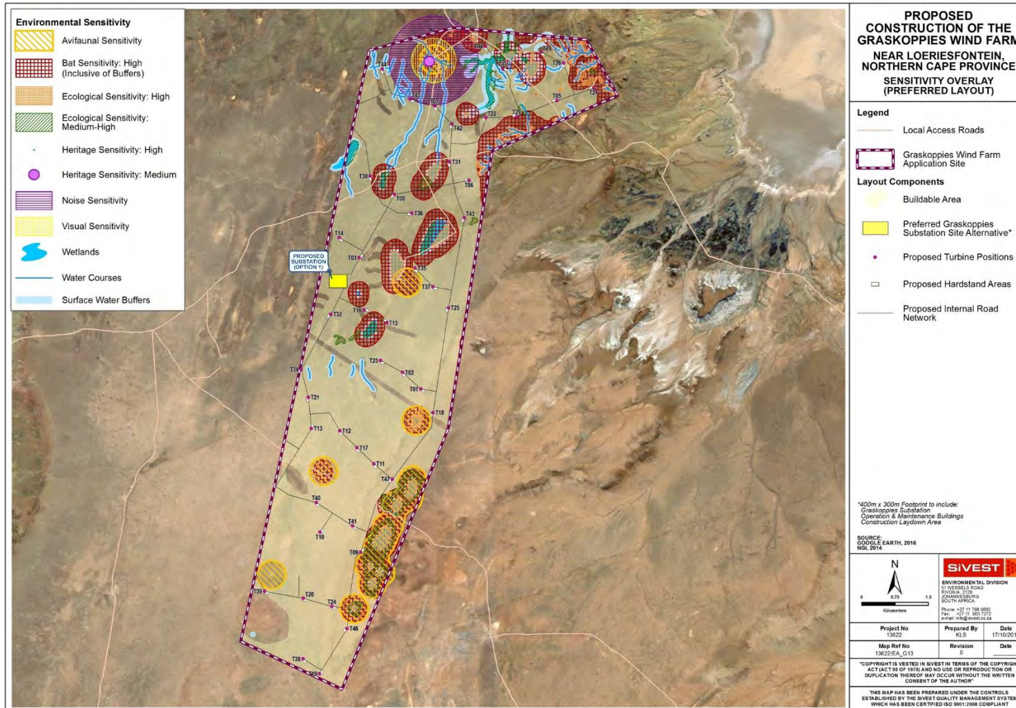
Figure 160: Preferred 47 Turbine Site Layout in relation to Sensitive Areas
