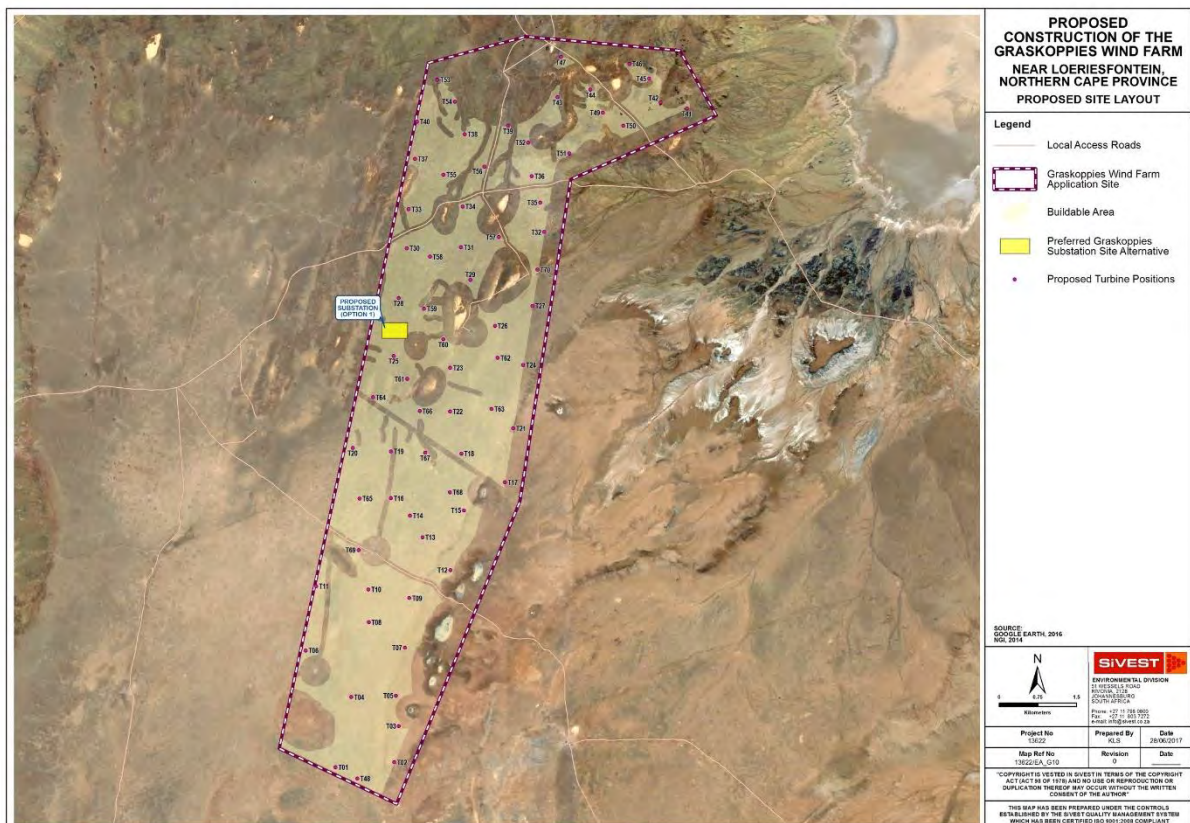
Figure 4: Proposed Graskoppies Layout
