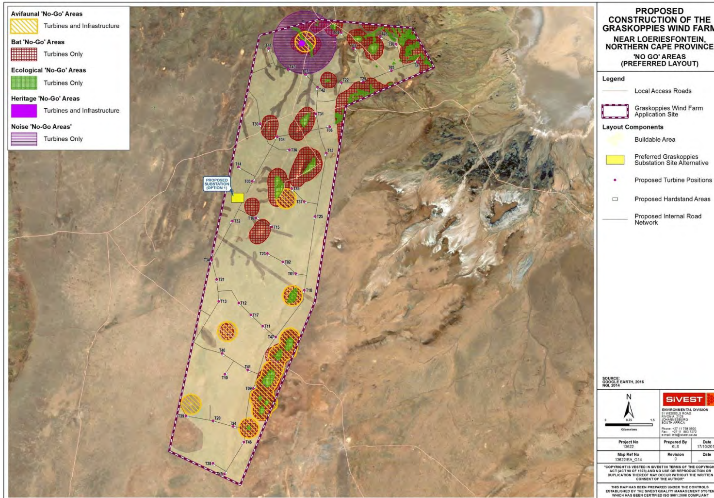
Figure 161: Preferred 47 Turbine Site Layout in relation to No-go Areas
