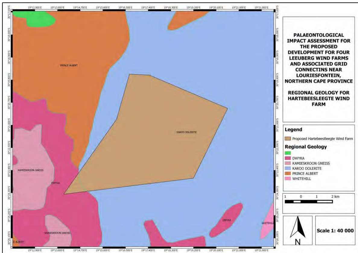
Figure 34: The surface geology of the proposed Hartebeest Leegte Wind Farm near Loeriesfontein in the Northern Cape Province. The development footprint is mostly underlain by Karoo Dolerite and a small area in the south west is underlain by the lowermost unit of the Karoo Supergroup, namely the Dwyka Group.
