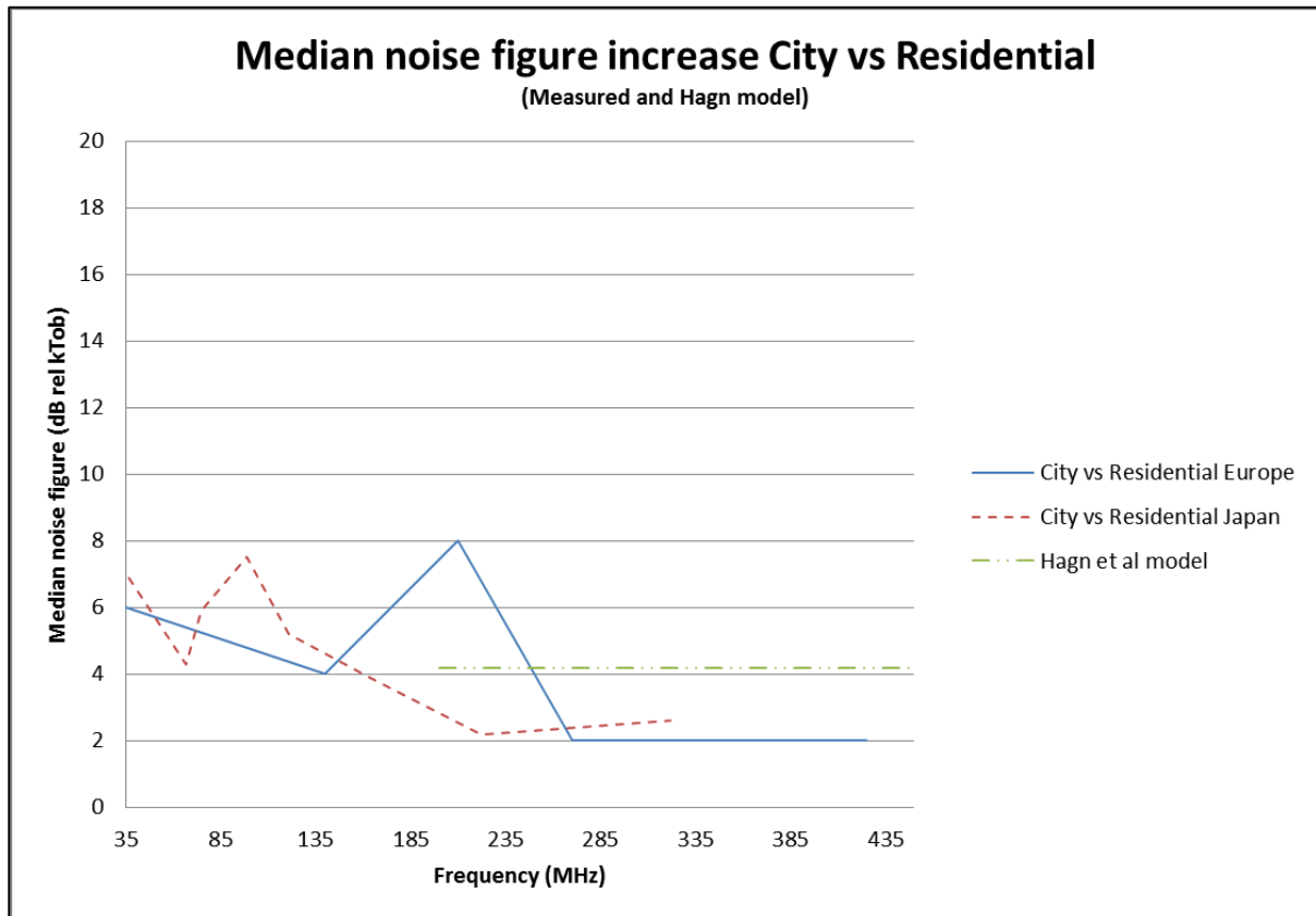
Figure 44: Man-made noise measured results (ITU-R P.372-13 Table 3 and Table 4, Hagn eq 8 and 9)
