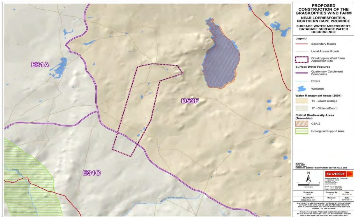
Figure 23: Database Surface Water Occurrence Map
