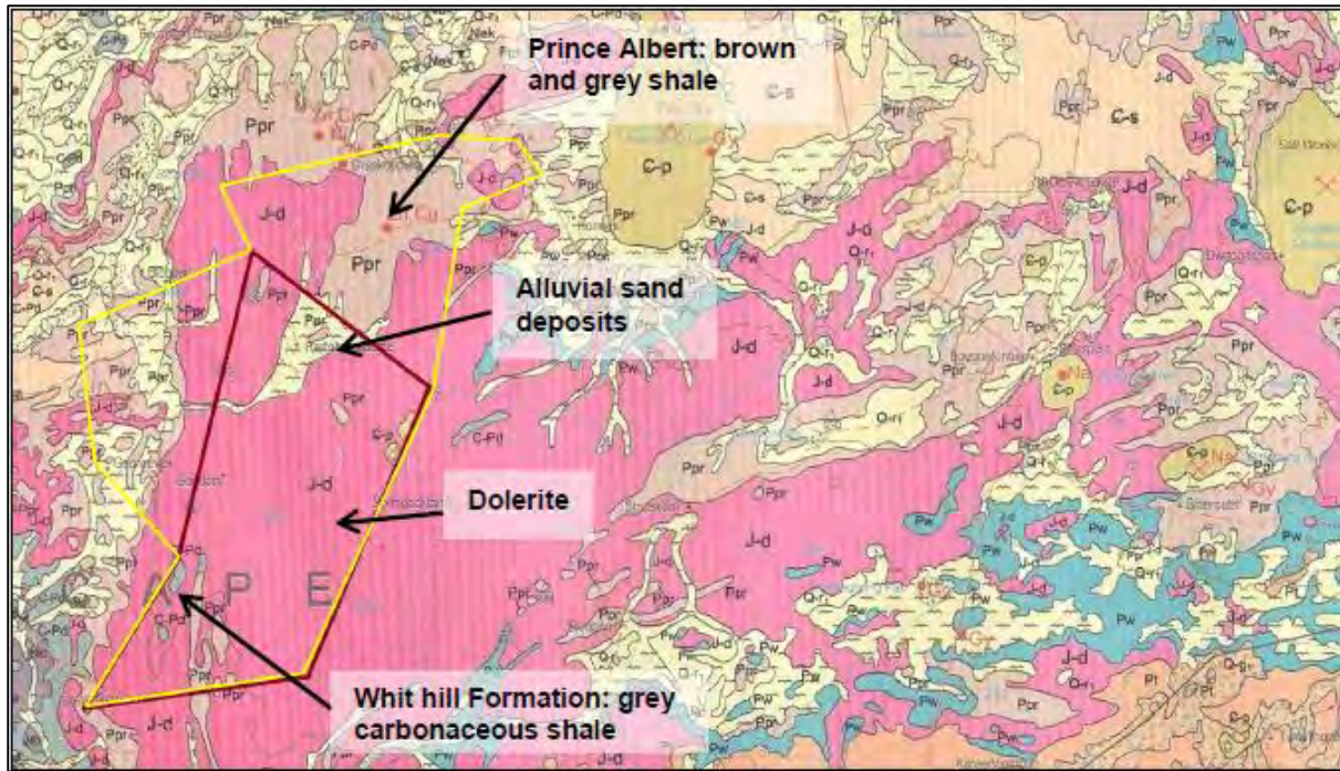
Figure 37: Extract from Loeriesfontein 2018 Geological Map
