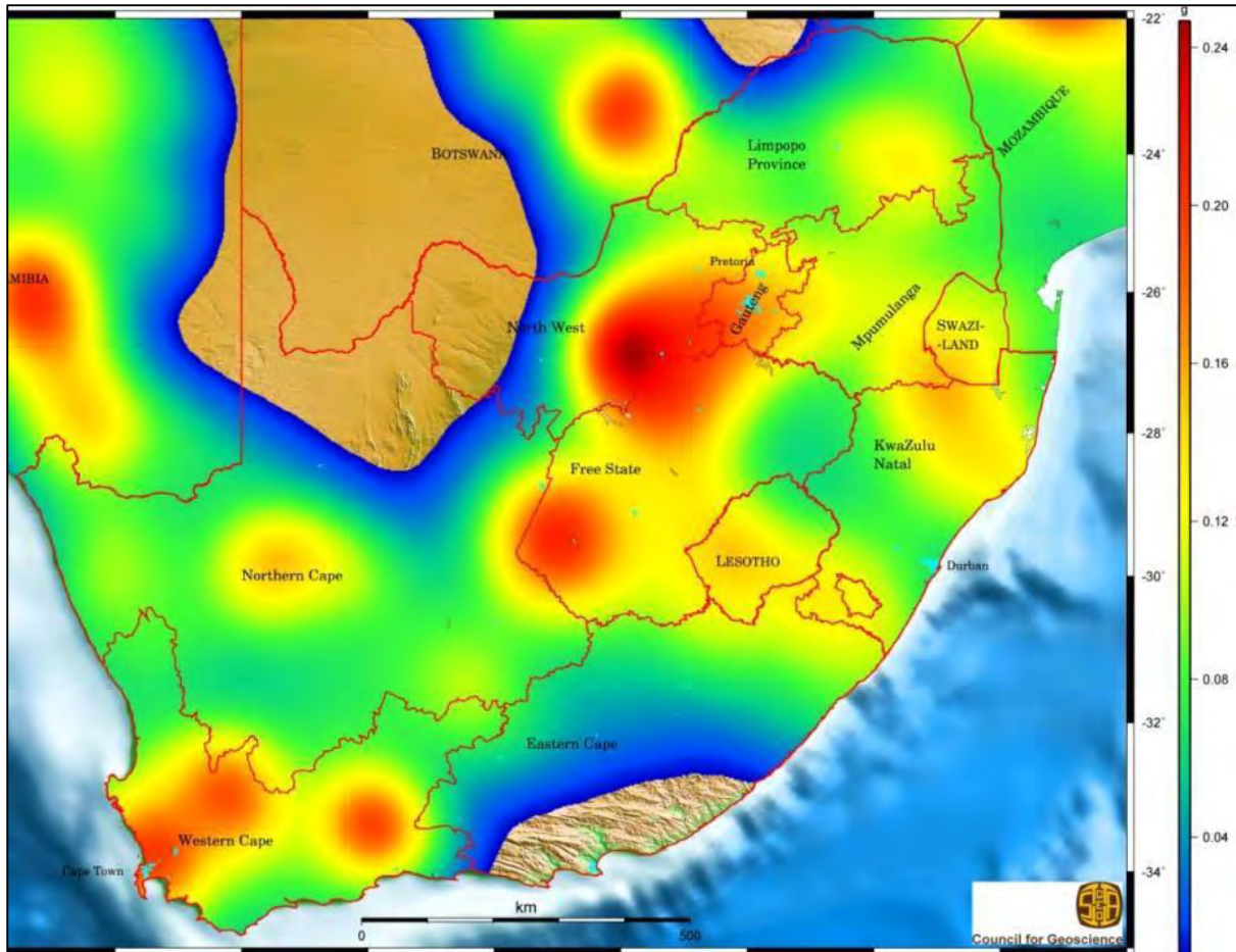
Figure 36: Seismic Hazard map of South Africa
