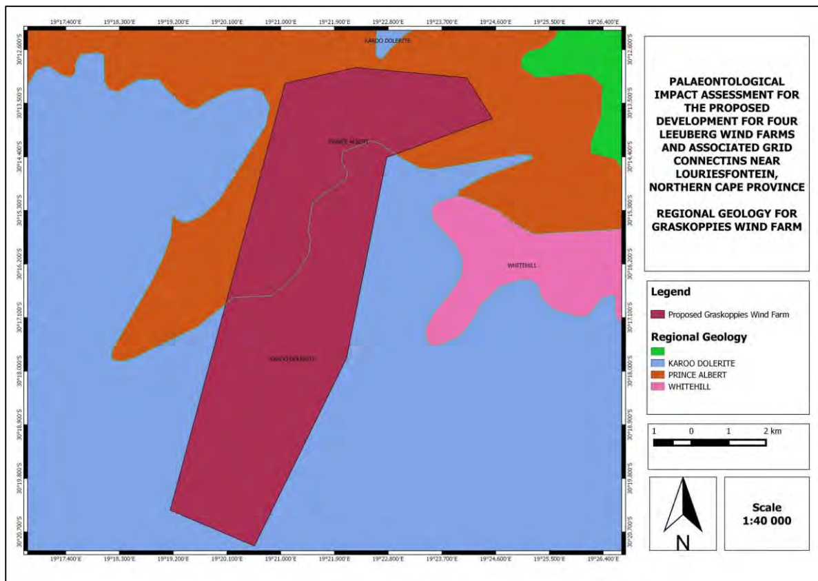
Figure 33: The surface geology of the proposed Graskoppies Wind Farm near Loeriesfontein in the Northern Cape Province. The development footprint is underlain by Karoo Dolerite as well as the Prince Albert and Whitehill Formations of the Ecca Group.
