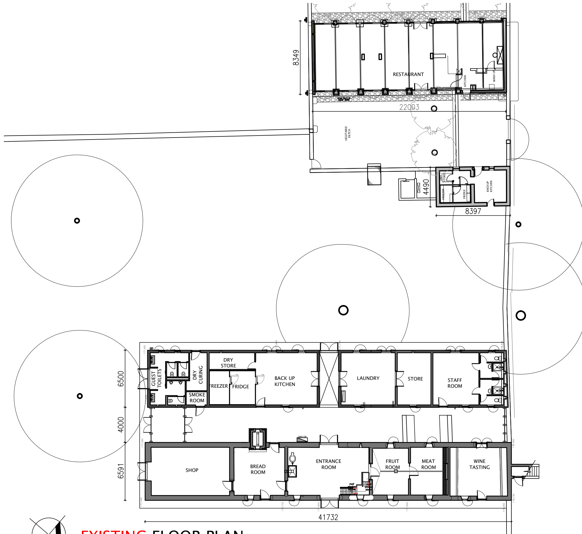
EXISTING FLOOR PLAN 1:250 @A3
