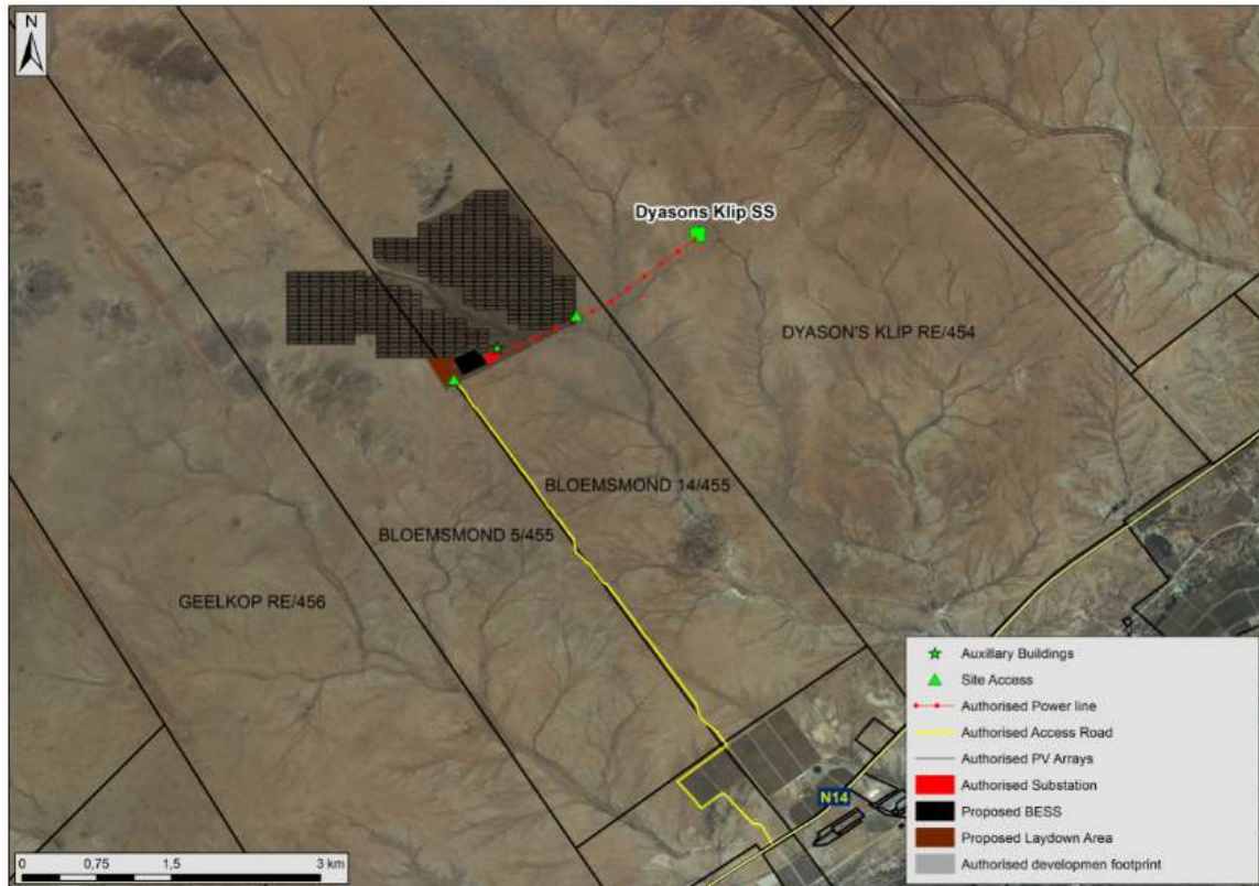
Figure 1. Proposed site layout plan for preferred development option (Bloemsmond PV 1)
