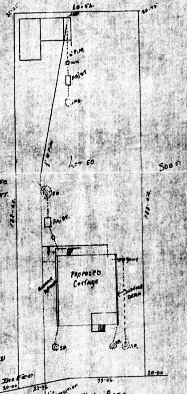
HAIG ROAD BLOCK PLAN SCALE 1" = 20 FT
