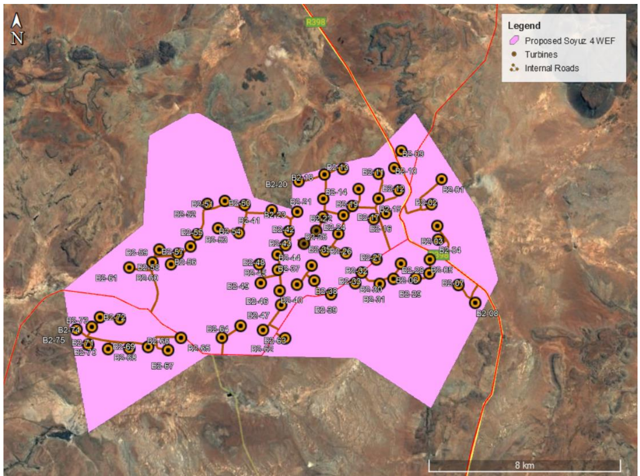
Figure 3-5: Internal roads
