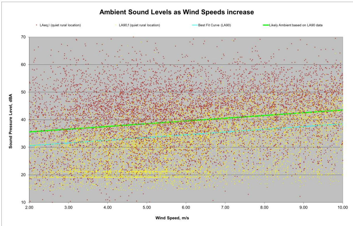
Figure 4-3: Ambient sound levels – quiet inland location (A-Weighted)
