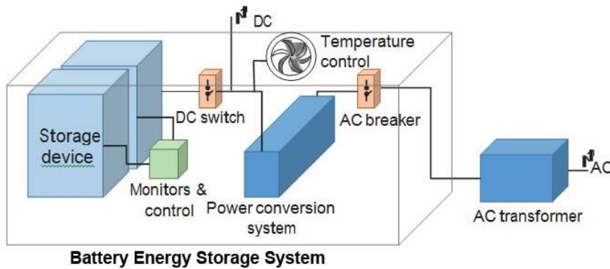
Figure 3-2: Conceptual BESS components 13
