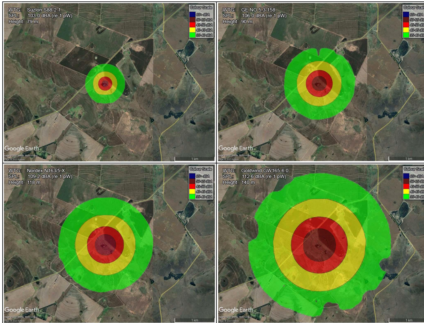
Figure 5-1: Extent of noises from different wind turbines (unmitigated, worst-case parameters)
