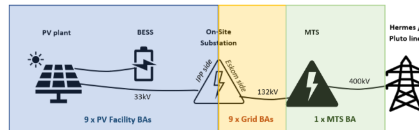
Figure 3-1: Components included in the individual BA processes for the Stilfontein Cluster
