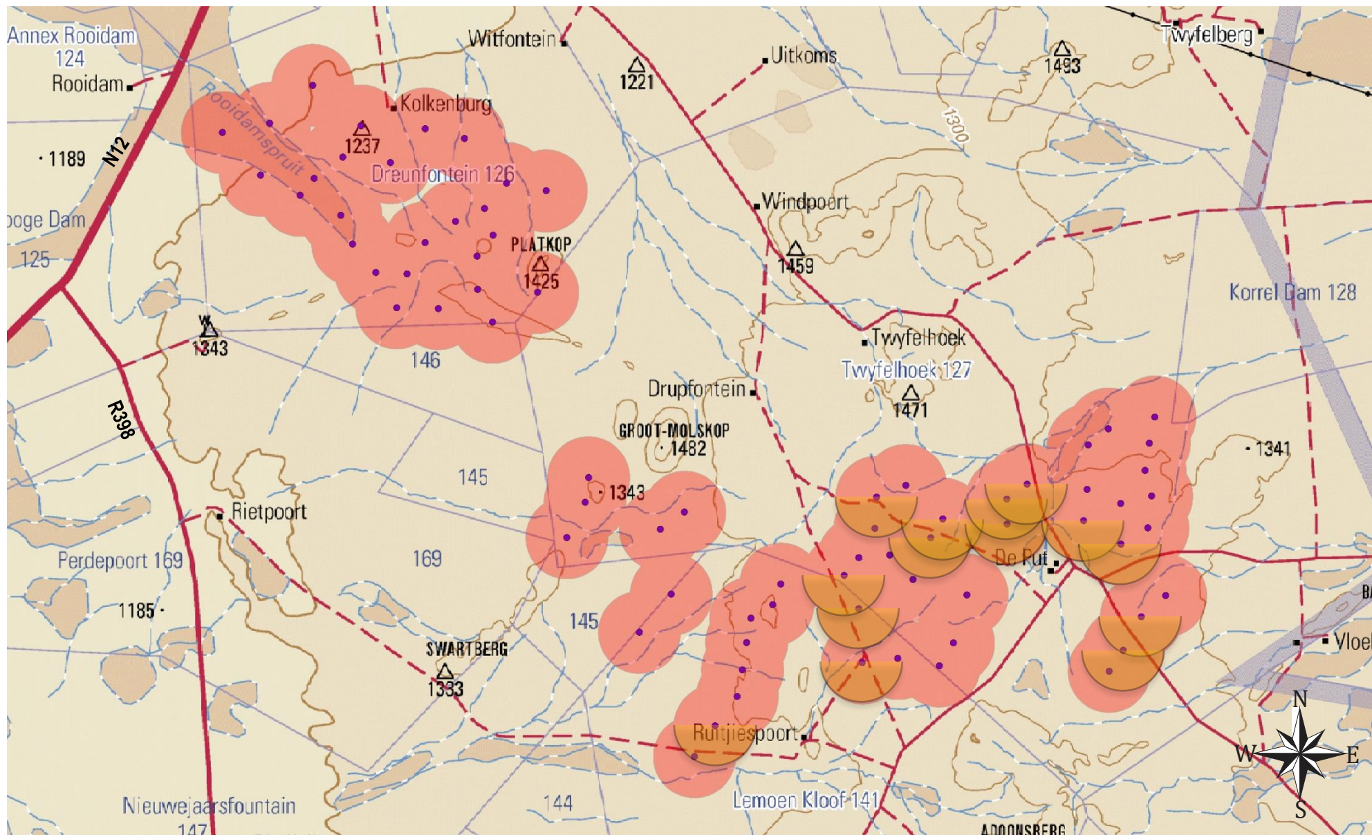
Map 9: Potential sensitive receptors exposed to shadow flicker from the proposed Soyuz 2 WEF
