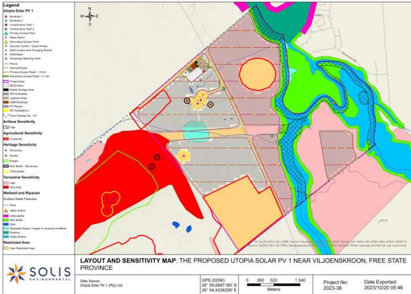
Figure 1: Environmental sensitivity map of the Utopia PV 1
