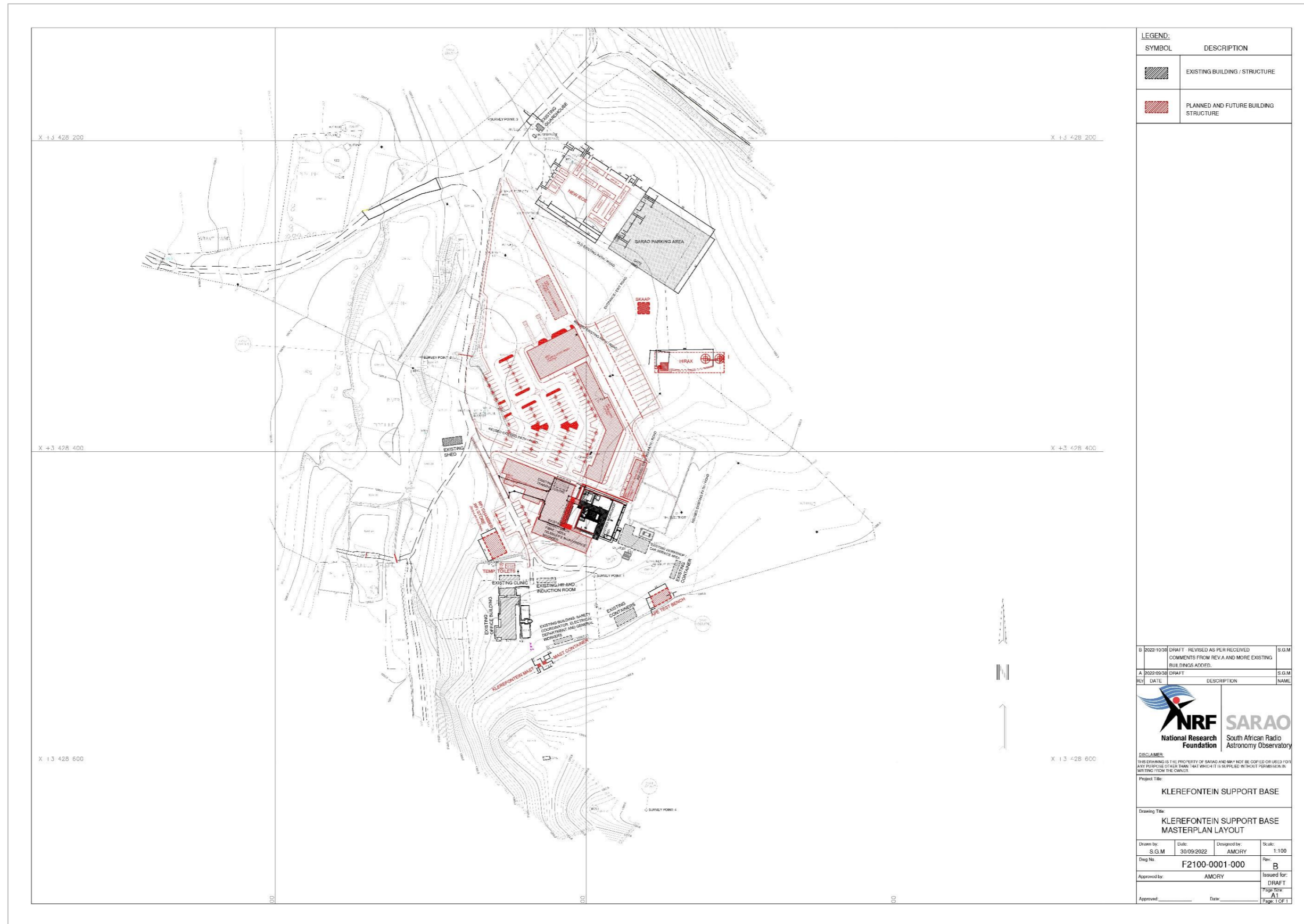
Figure 8-1: Klerefontein Support Base Masterplan Layout
