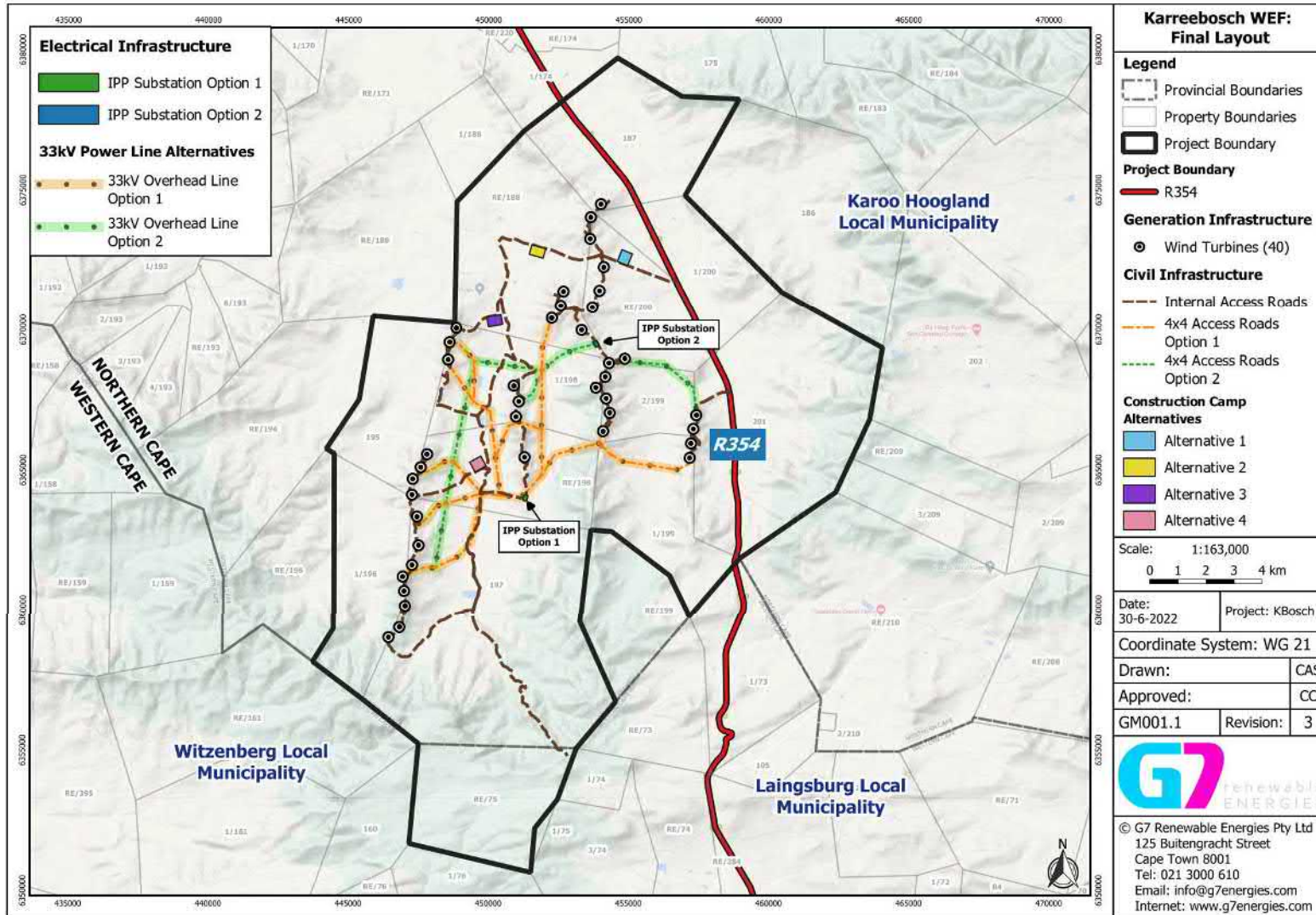
Figure 1: Proposed Final Layout of the Karreebosch WEF and Associated Infrastructure Produced by G7 Renewable Energies
