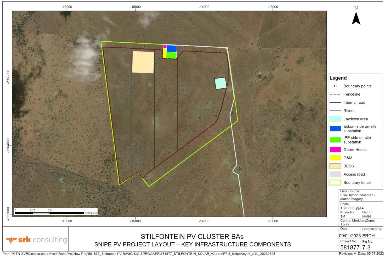
Figure 1-5: Snipe PV project layout – key infrastructure components 3
