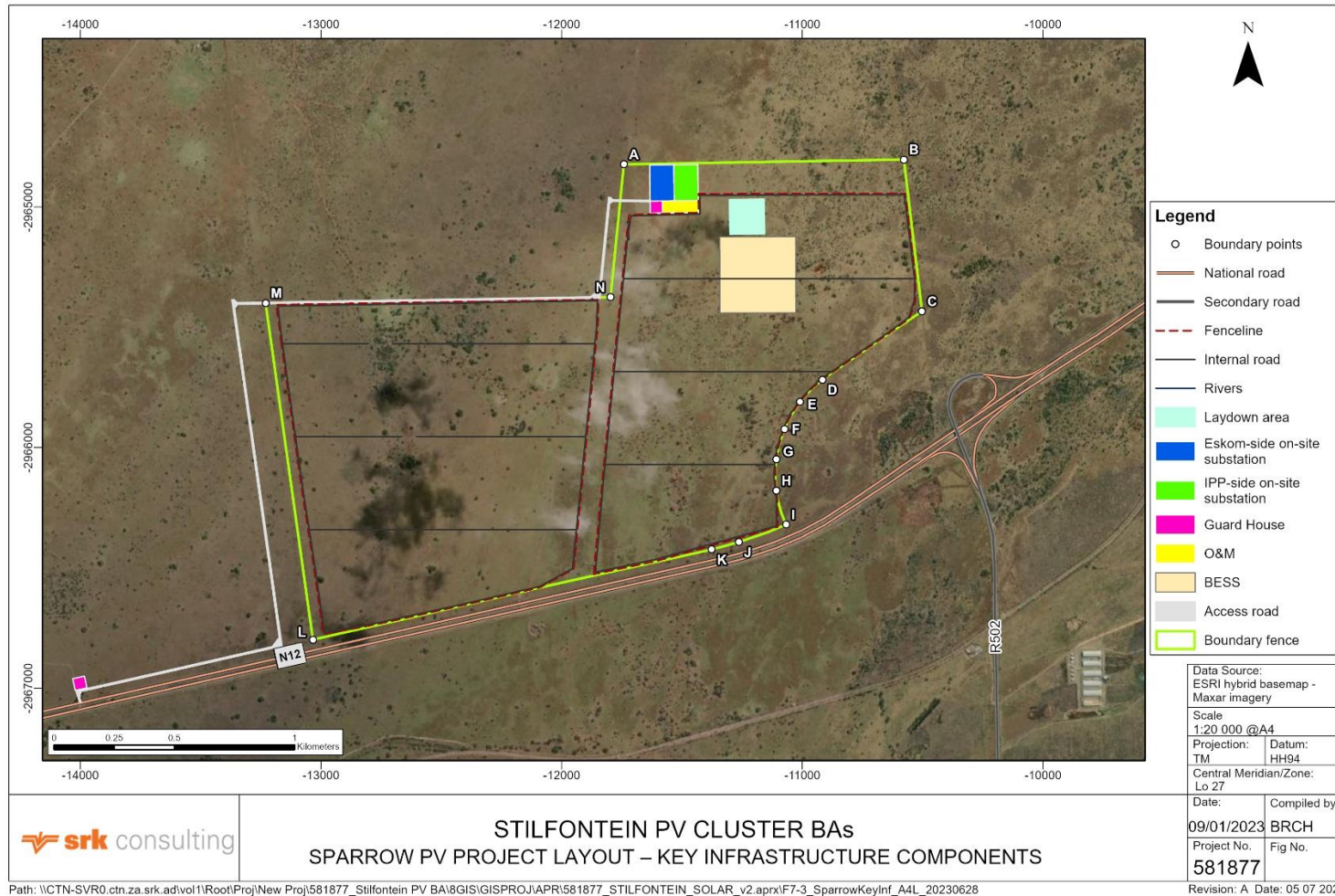
Figure 1-5: Sparrow PV project layout – key infrastructure components 3
