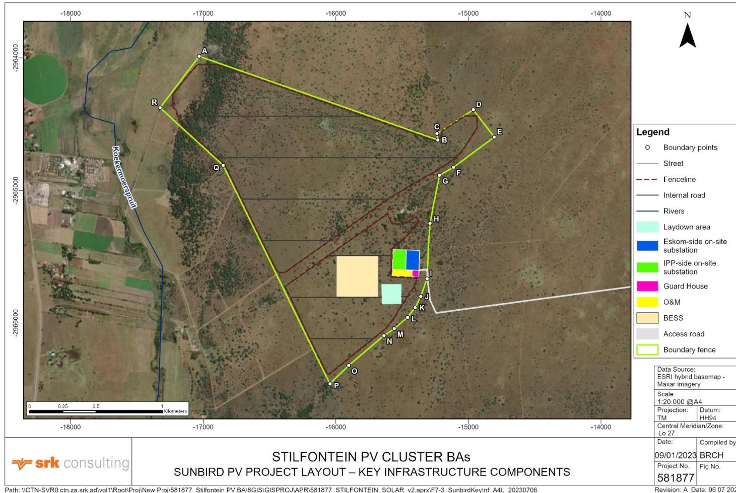
Figure 1-5: Sunbird PV project layout – key information components 3
