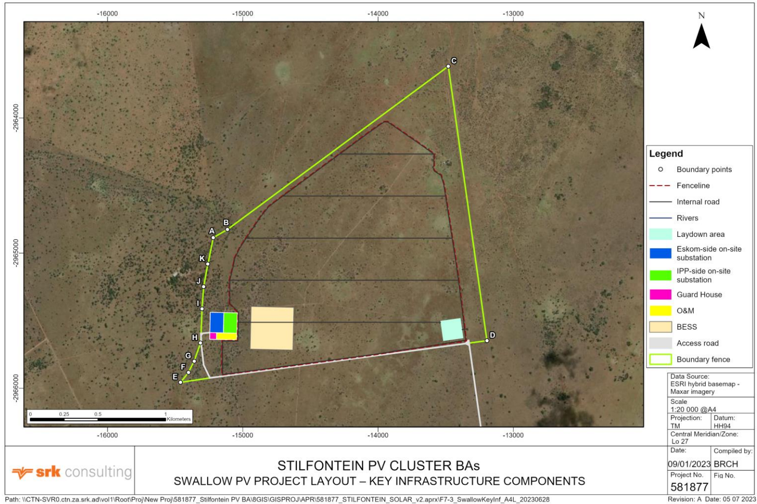
Figure 1-5: Swallow PV project layout - key infrastructure components 3
