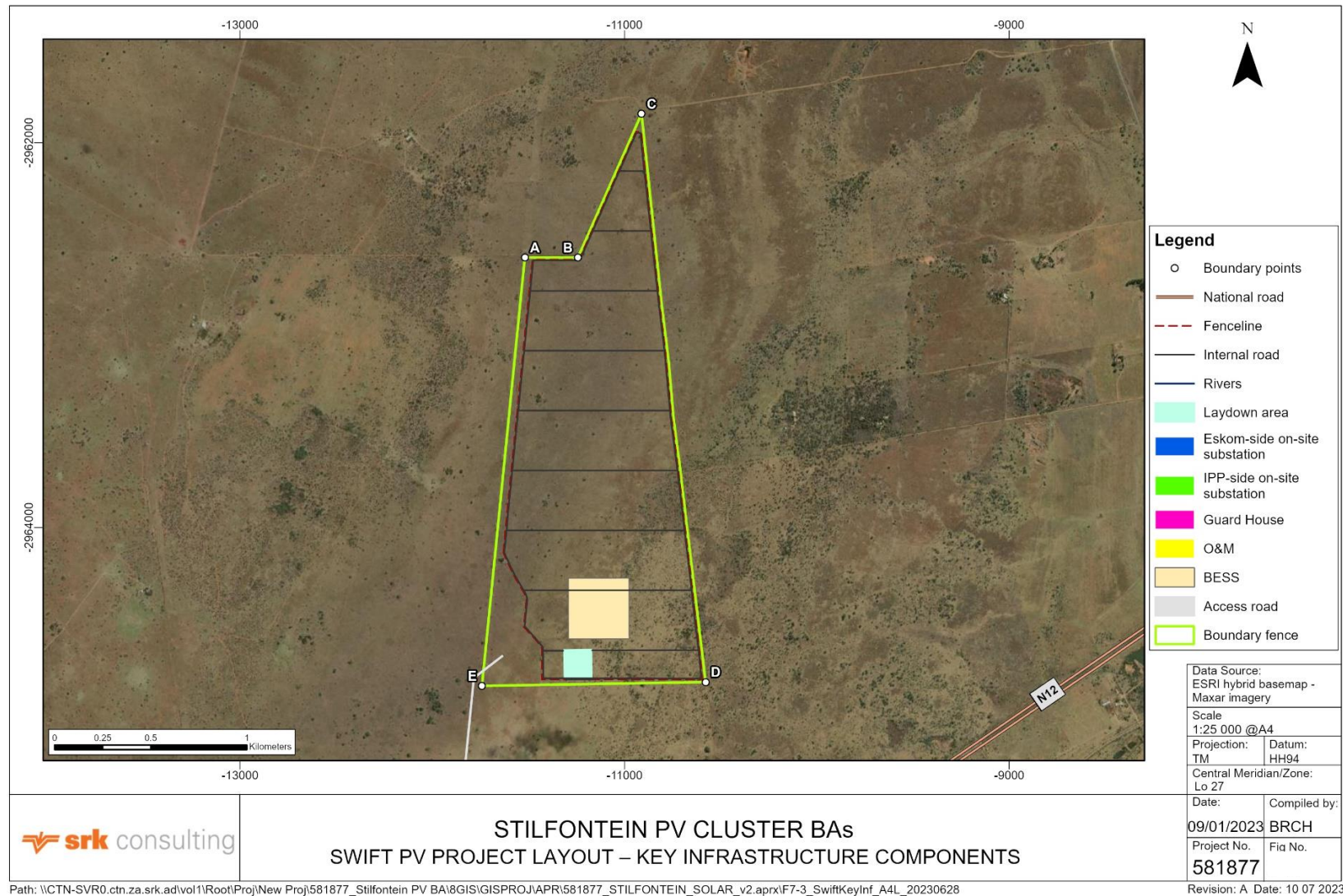
Figure 1-5: Swift PV project layout – key infrastructure components 3
