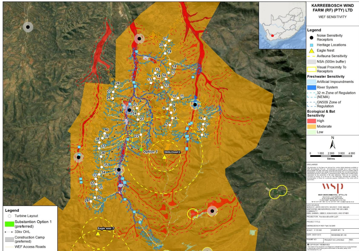
Figure 1.3: Environmental sensitivity map overlain over the Final Karreebosch WEF Layout
