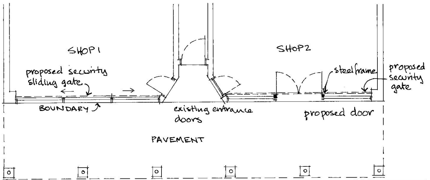
PART PLAN
