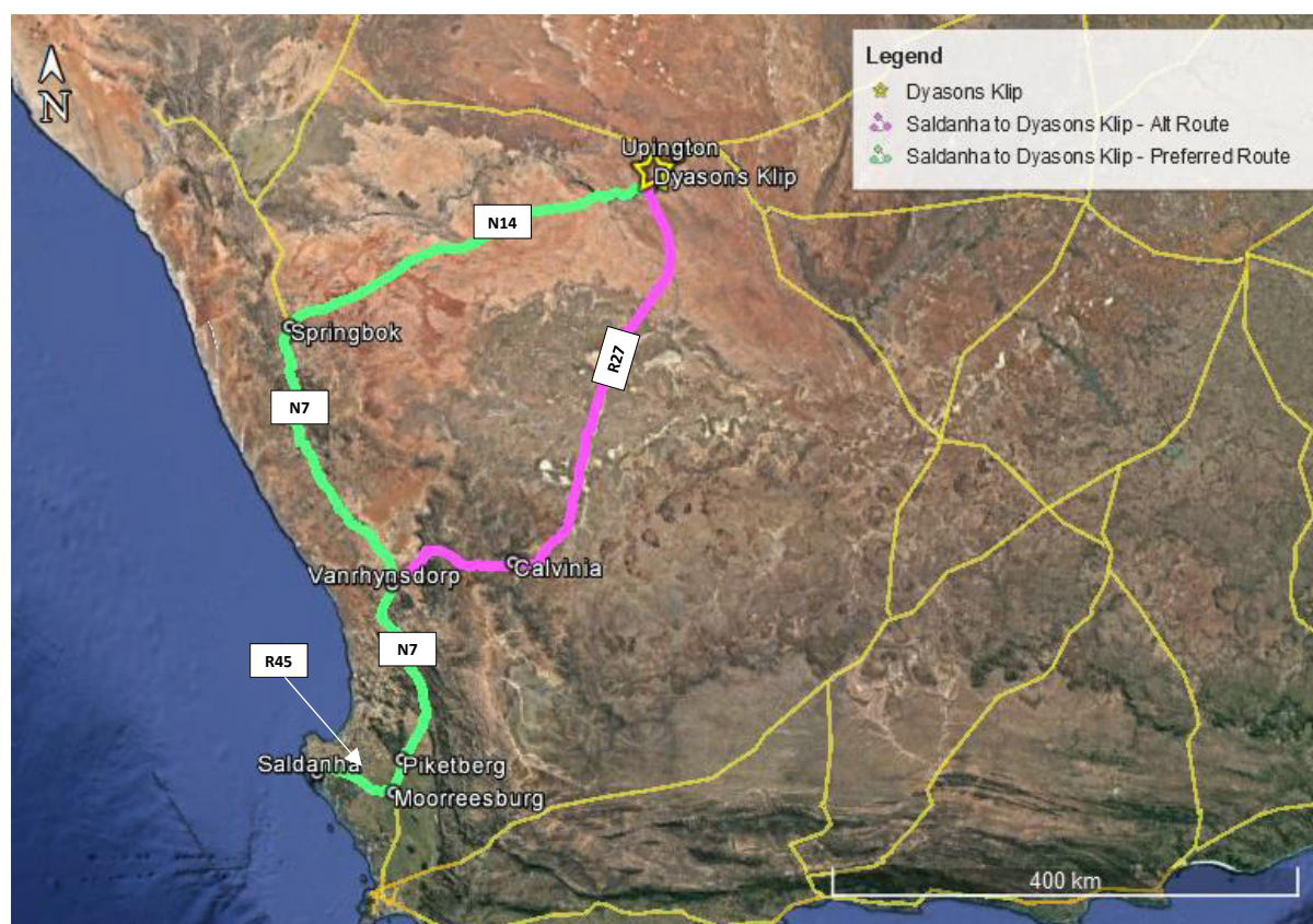
Figure 2-1: Haulage Routes (Port of Entry - Saldanha)
