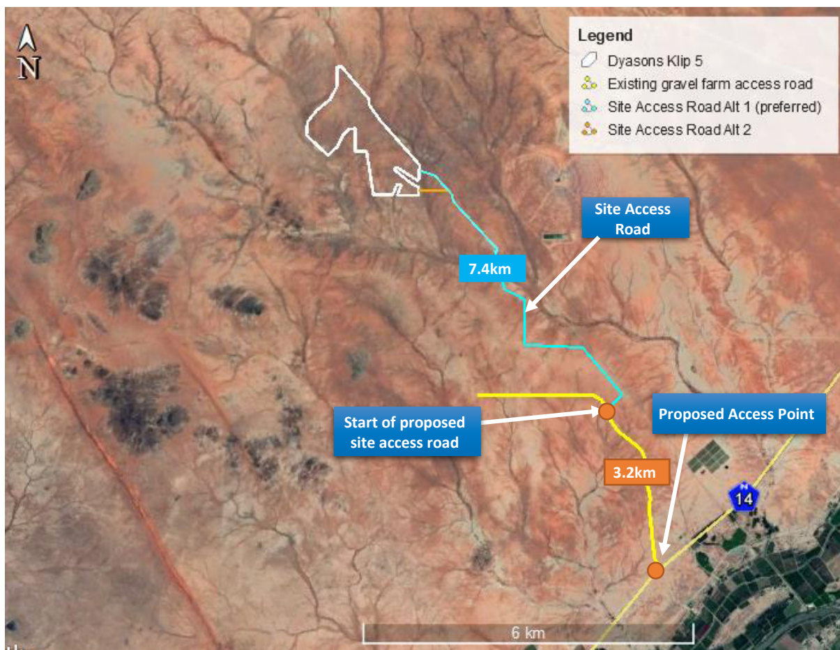
Figure 3-7: Aerial View of the Access Point, Existing Gravel Road and New Access Road
