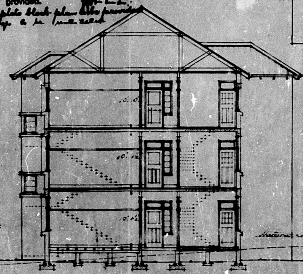
CROSS SECTION I
