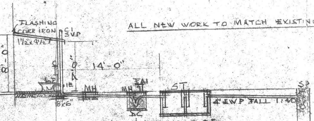
SECTION OF VC & DRAINAGE
