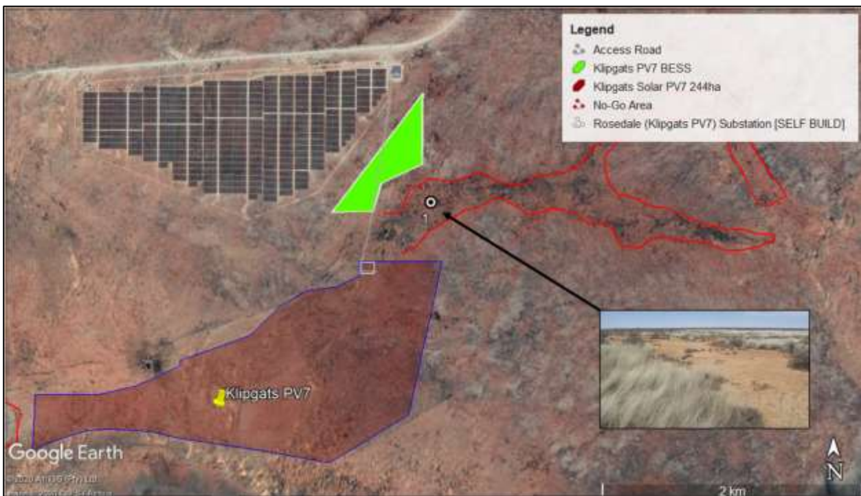
Spatial layout of proposed BESS in relation to previously delineated No-Go areas (red)
