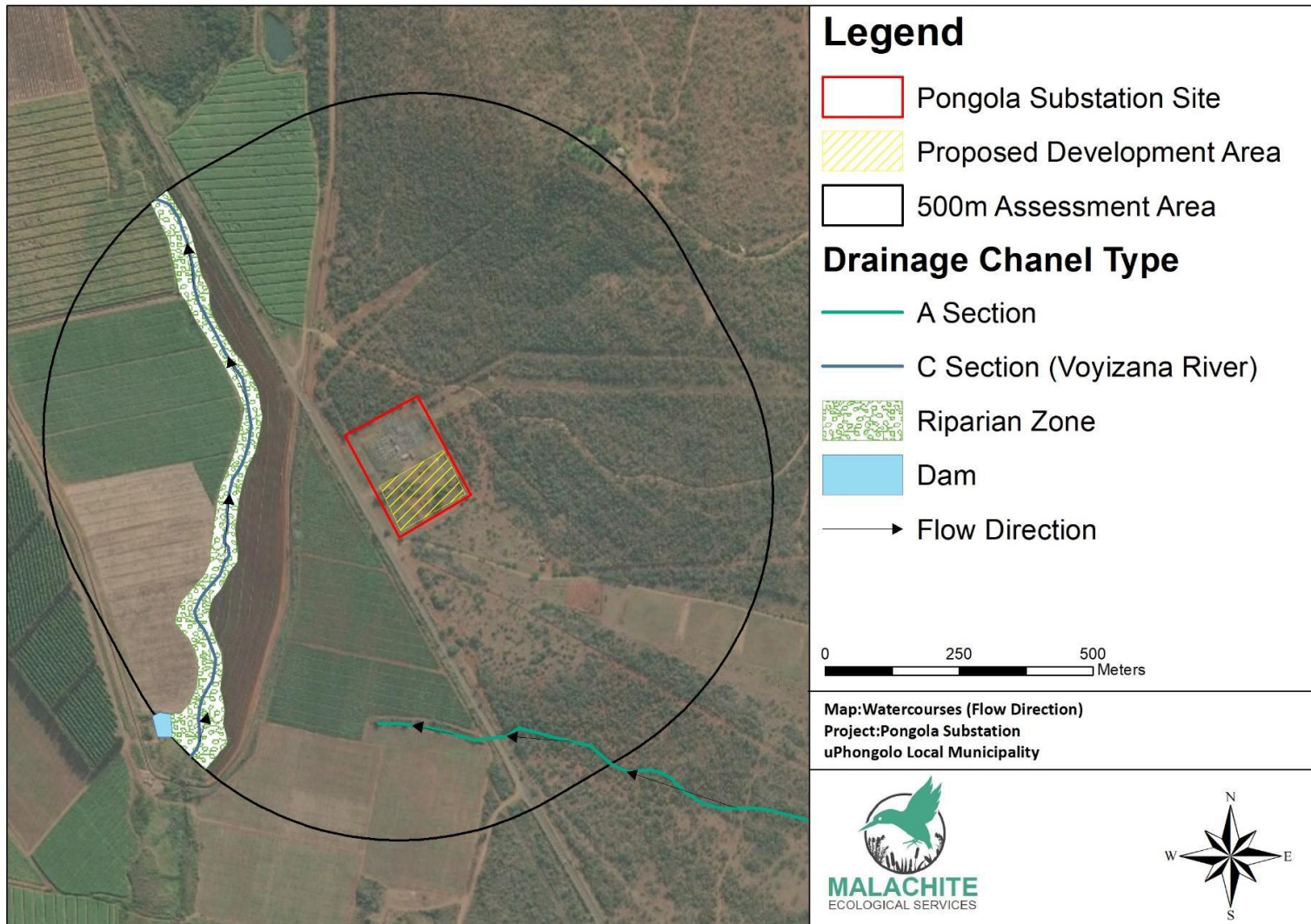
Figure 13: Flow Direction of the Identified Watercourses (Malachite Wetland Assessment, 2019)
